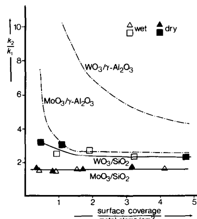
FIG. 5. Ratio between reaction rate constants from the hydrogenation of butene and the hydrodesulfurization of thiophene, k_2/k_1 , as a function of the average surface coverage, for sulfided \text{MoO}_3/\text{SiO}_2 , \text{WO}_3/\text{SiO}_2 , \text{MoO}_3/\gamma\text{-Al}_2\text{O}_3 , and \text{WO}_3/\gamma\text{-Al}_2\text{O}_3 catalysts, prepared by dry and wet impregnation (data for alumina-based catalysts are presented in Ref. (1)).
