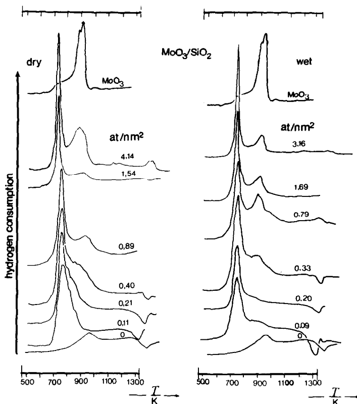
FIG. 1. TPR patterns of \text{SiO}_2 , \text{MoO}_3 , and \text{MoO}_3/\text{SiO}_2 catalysts prepared by dry and wet impregnation.
