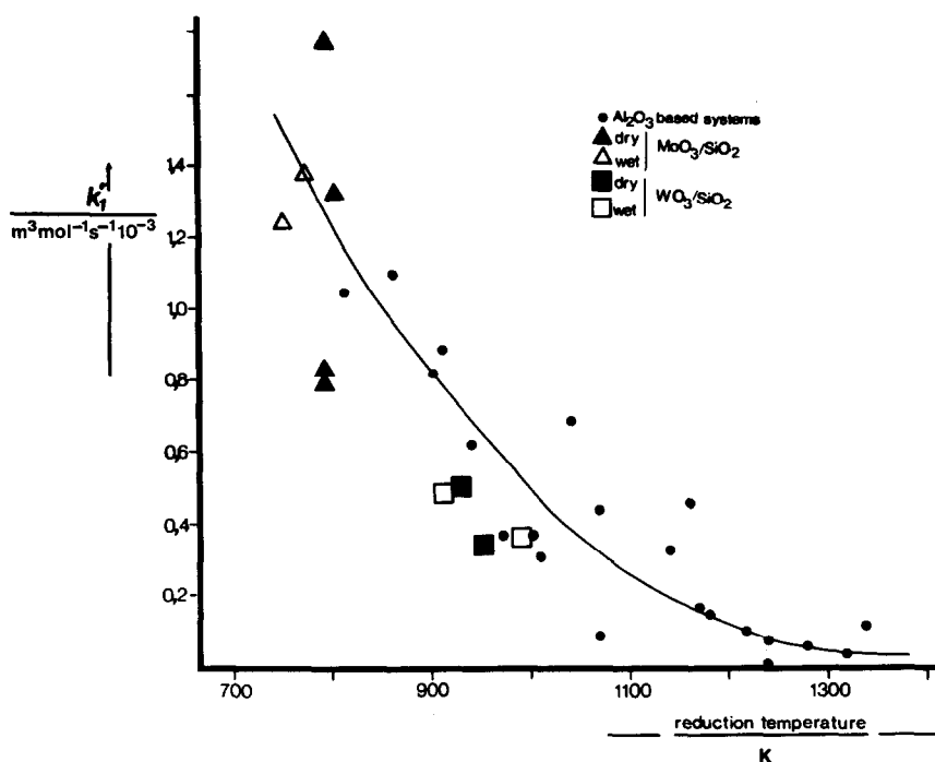
FIG. 6. Relation between the reaction rate constant k_i for hydrodesulfurization of thiophene of sulfided \text{MoO}_3/\text{SiO}_2 , \text{WO}_3/\text{SiO}_2 , \text{MoO}_3/\gamma\text{-Al}_2\text{O}_3 , and \text{WO}_3/\gamma\text{-Al}_2\text{O}_3 catalysts and the average reduction temperature (data for alumina-based catalysts are presented in Ref. (1)).
