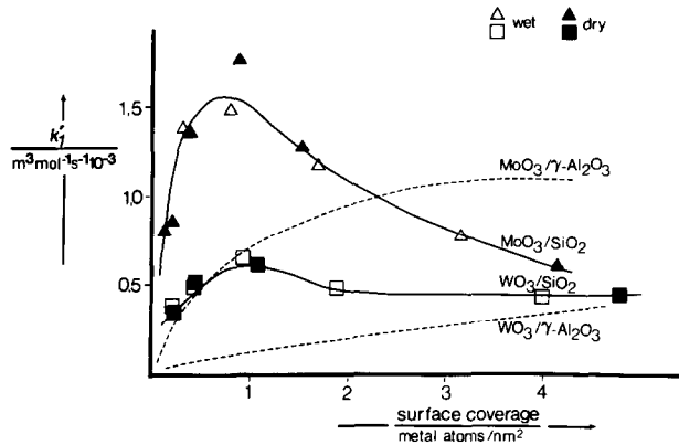
FIG. 3. Reaction rate constant k_1' for the hydrodesulfurization of thiophene as a function of the average surface coverage for sulfided \text{MoO}_3/\text{SiO}_2 , \text{WO}_3/\text{SiO}_2 , \text{MoO}_3/\gamma\text{-Al}_2\text{O}_3 , and \text{WO}_3/\gamma\text{-Al}_2\text{O}_3 catalysts prepared by dry and wet impregnation (data for alumina-based catalysts are presented in Ref. (1)).
