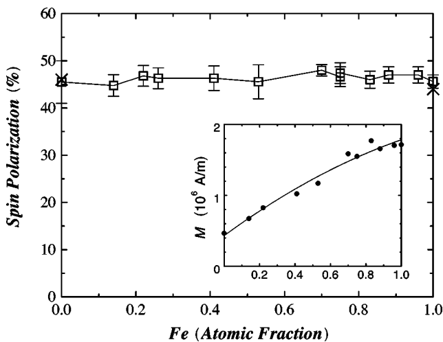
FIG. 2. PCAR results for the spin polarization P as a function of Fe content for \text{Ni}_x\text{Fe}_{1-x} samples. ( \square ), films; ( \times ), pure Ni and Fe foils and single crystals. Inset: Magnetic moment, M , as a function of the Fe content for \text{Ni}_x\text{Fe}_{1-x} samples. The lines are guides to the eye.
