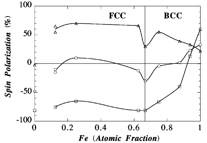
FIG. 3. The results of the band-structure calculations for P_N , P_{NV} , and P_{NV^2} : ( \square ), P_N ; ( \circ ), P_{NV} ; ( \triangle ), P_{NV^2} . The lines are guides to the eye. The results for pure Ni are shown for completeness.
