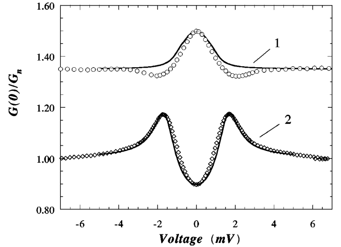
FIG. 1. G(V)/G_n as a function of voltage V for two samples: 1 ( \circ ), Fe point/Ta foil base; 2 ( \diamond ), Nb point/ \text{Ni}_{80}\text{Fe}_{20} film base; solid curves—modified BTK fits ( T=1.7 K, Z=0 , \Delta=0.6 meV and T=2.2 K, Z=0.4 , \Delta=1.5 meV, respectively). The values of P obtained from these fits are 42.5% for Fe and 49.5% for \text{Ni}_{80}\text{Fe}_{20} . Note that the bath temperature in the latter case was 1.8 K (see text). Curve 1 has an arbitrary vertical offset.
