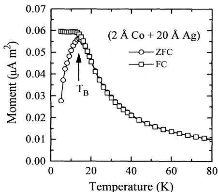
FIG. 8. Field-cooled (FC) and zero-field-cooled (ZFC) magnetization measured in a field of 50 Oe applied parallel to the film plane for the sample 100 \times (2 \text{ \AA Co} + 20 \text{ \AA Ag}) . The maximum in the ZFC curve occurs at 15 K.
