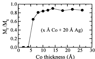
FIG. 9. Remanent in-plane magnetization of the 100 \times (x \text{ \AA Co} + 20 \text{ \AA Ag}) multilayers.
