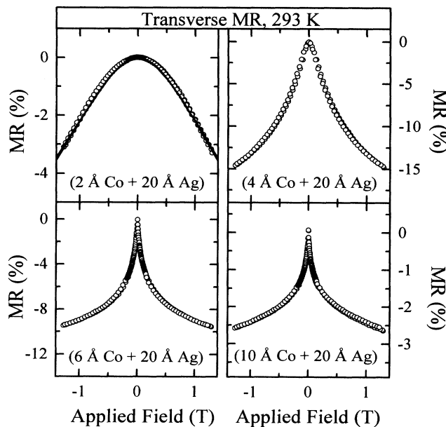
FIG. 11. Field dependence of the magnetoresistance with the applied field parallel to the film plane for ( x Co+20 Å Ag) multilayers with nominal Co thicknesses of 2, 4, 6, and 10 Å. The magnetoresistance is defined as (R_{B=0}-R_{B=1.3\text{ T}})/R_{B=0} and was measured at room temperature. Note the differences in the scales of the y axes [magnitude of the MR (%)]. The MR data of the multilayer with 2 Å Co are compared with the function -A(M/M_s)^2 with A=0.16 (solid line).
