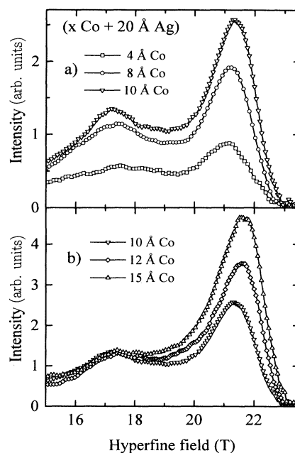
FIG. 2. NMR spectra of the as-deposited ( x \text{ \AA} \text{ Co} + 20 \text{ \AA} \text{ Ag} ) multilayers for various nominal Co thicknesses. The integrals (between 15 and 23 T) of the spectra are normalized to the nominal Co thickness. The spectra are corrected for enhancement.
