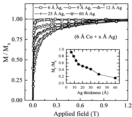
FIG. 10. Field dependence of the magnetization of the 100 \times (6 \text{ \AA Co} + x \text{ \AA Ag}) multilayers for nominal Ag thicknesses between 6 and 60 Å. The measurements were performed at room temperature with the applied field parallel to the film plane. The inset shows the remanent magnetization as a function of the Ag spacer-layer thickness.
