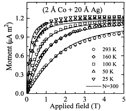
FIG. 6. Field dependence of the magnetization of the sample 100 \times (2 \text{ \AA} \text{ Co} + 20 \text{ \AA} \text{ Ag}) measured at various temperatures between 25 and 293 K with the applied field parallel to the film plane.
