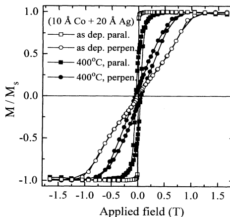
FIG. 16. Influence of annealing on the in-plane (squares) and perpendicular (circles) magnetization of the sample 100 \times (10 Å Co + 20 Å Ag). The as-deposited data are given by the open symbols, whereas the closed symbols represent the data after annealing at 400°C. The measurements were performed at room temperature.
