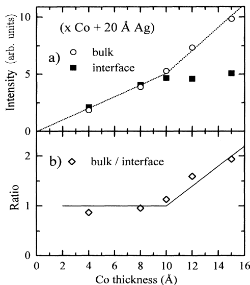
FIG. 3. Intensity of the interface part (a), the bulk part (a), and the ratio between the bulk and the interface part (b), as derived from Fig. 2, as a function of the nominal Co thickness. The dotted line in (a) is a guide to the eye; the solid line in (b) is in accordance with the model discussed in the text.
