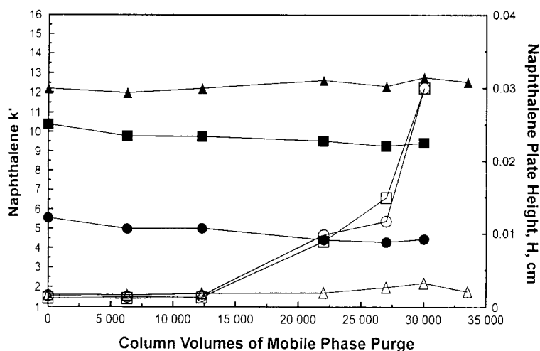
Fig. 7. Effect of stationary type on column ageing at pH 9. Columns: 15 × 0.46 cm I.D. Zorbax SB-C 8 (diisopropyl-C 8 , ○), Zorbax SB-C 18 (diisobutyl-C 18 , □) and Zorbax Rx-C 18 (dimethyl-C 18 , Δ); open symbols, H ; solid symbols, k' ; conditions as in Fig. 6.
