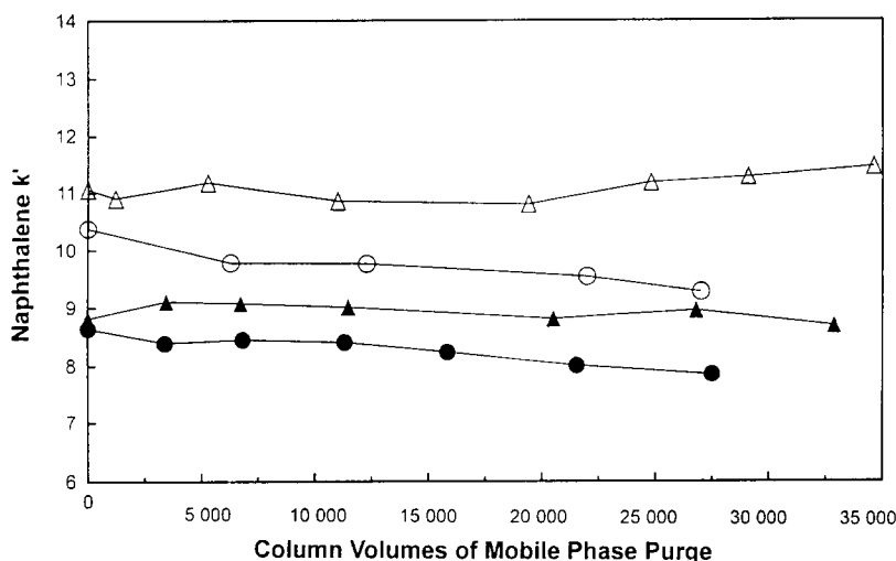
Fig. 8. Effect of organic modifier on k' for column ageing at pH 9: naphthalene solute. Columns: 15 × 0.46 cm I.D. Zorbax SB-C 18 (diisobutyl-C 18 , ○) and Zorbax Rx-C 18 (dimethyl-C 18 , Δ); mobile phase purge: methanol-0.01 M phosphate, pH 9.0 (60:40); flow-rate: 1.0 ml/min; solute: naphthalene; ambient temperature. Open symbols, methanol; closed symbols, acetonitrile.
