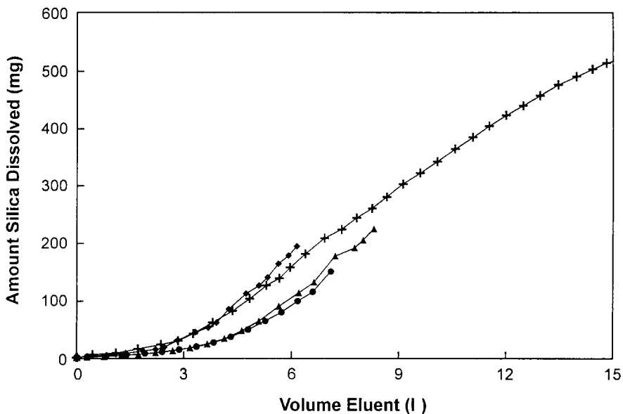
Fig. 4. Effect of bonded stationary phase type on silica support dissolution: methanol modifier. Columns: 15 \times 0.46 cm I.D., (●) Zorbax-ODS (dimethyl- C_{18} ; Type A silica), (▲) Zorbax Rx- C_{18} (dimethyl- C_{18} ; Type B silica), (◆) Zorbax SB- C_{18} (diisobutyl- C_{18} ; Type B silica) and (+) Zorbax SB- C_8 (diisopropyl- C_8 ; Type B silica); conditions of Fig. 1, except methanol-pH 10 buffer mobile phase.
