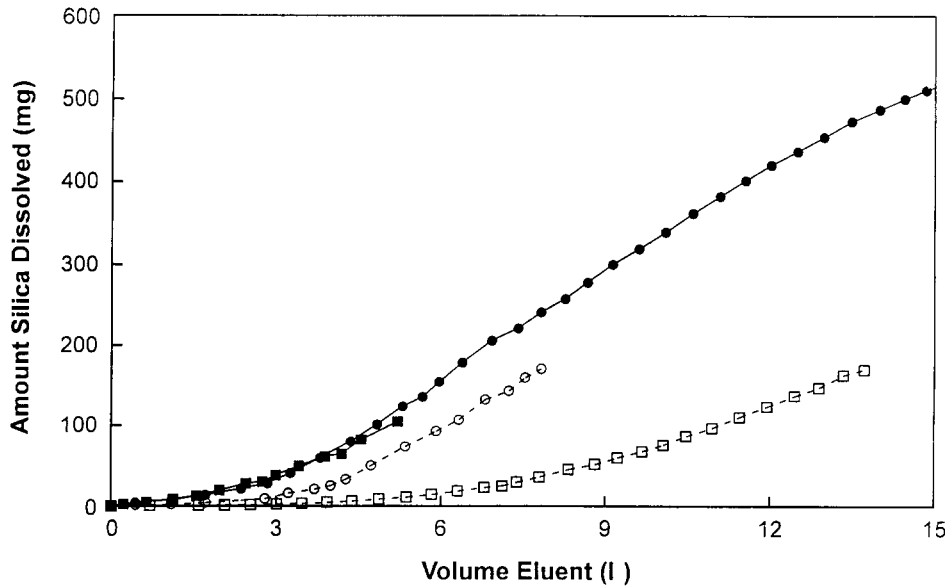
Fig. 2. Silica support dissolution for diisopropyl- C_{18} column. Columns: 15 \times 0.46 cm I.D. Zorbax SB- C_8 (diisopropyl- C_8 ; solid symbols) and Zorbax Rx- C_{18} (dimethyl- C_{18} ; open symbols); same mobile phases and pH 10 buffer conditions as in Fig. 1. \circ = Methanol, \square = acetonitrile.
