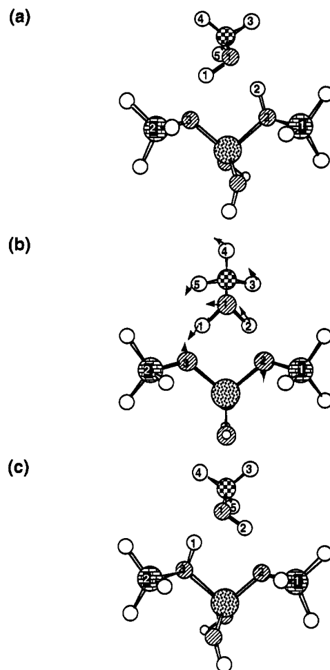
Figure 1. Hydrogen exchange: adsorption (a) and dissociative (c) complexes and TS (b).
