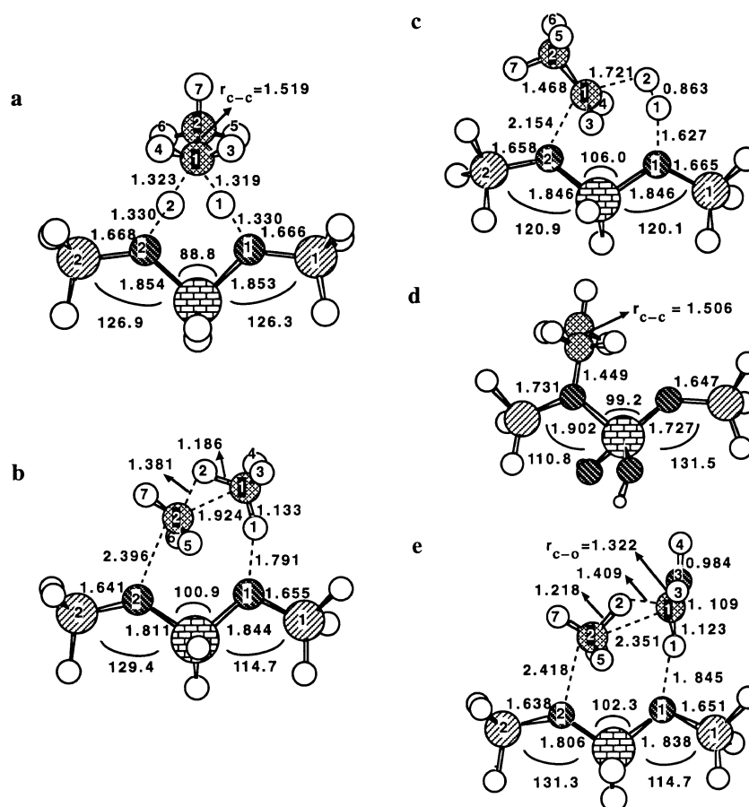
Fig. 2. Transition states for (a) hydrogen exchange, (b) cracking, and (c) dehydrogenation of ethane, (d) surface ethoxy species and (e) TS for hydride transfer between methanol and a surface methoxy species. All structures were obtained with DFT/DZVP including nonlocal corrections at the end of the optimization. Distances in Å and angles in deg. See fig. 1 for the pattern of the atoms. (The pictures (a)–(c) and (e) are reprinted from ref. [19], copyright 1996 American Chemical Society.)
