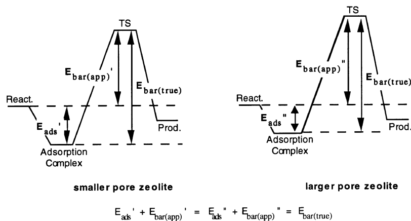
Fig. 3. The relation between the apparent activation energy, E_{\text{bar(app)}} , and the adsorption energy of the molecule, E_{\text{ads}} , for a first-order reaction of two different zeolites with same intrinsic acidity.
