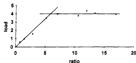
Figure 2. Number of Bengal Rose molecules encapsulated in one dendritic box as determined by UV-vis spectroscopy versus the molar ratio of Bengal Rose and dendrimer during the encapsulation reaction (using 10^{-3} M poly(propylene imine) dendrimer in \text{CH}_2\text{Cl}_2 ).
