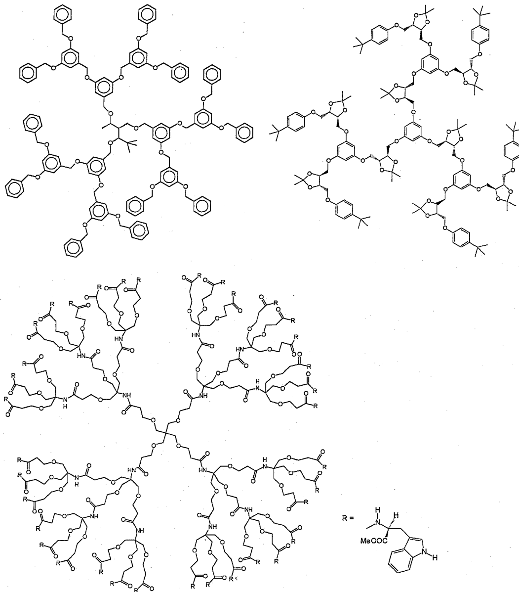
Figure 1. A selected anthology of chiral dendrimers and their classification. Top left: class 1 Seebach's dendrimer with a chiral core [4]. Top right: class 2 Chow's dendrimer with chiral building blocks [5]. Bottom class 3, Newkome's dendrimers with chiral end groups [6].
