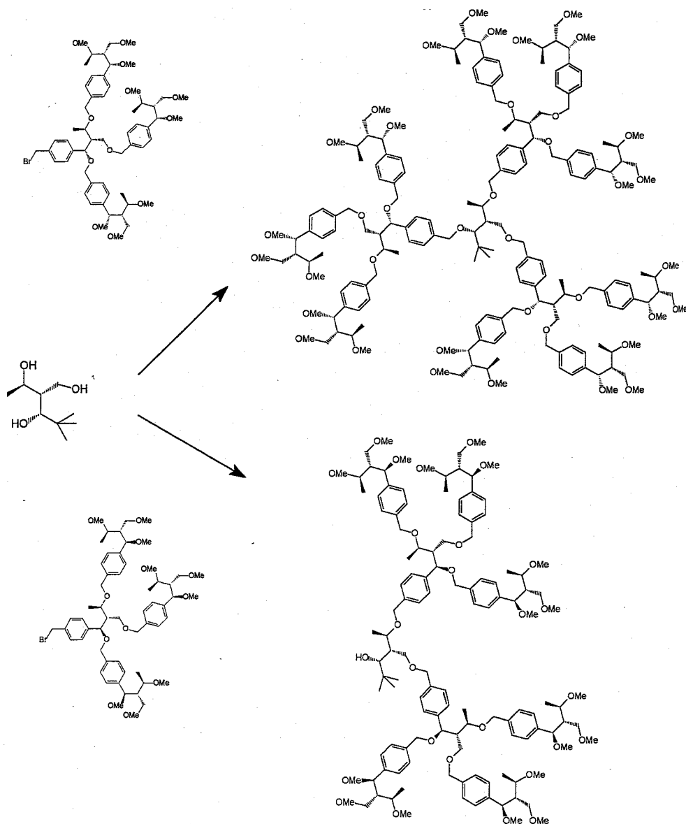
Figure 11. Diastereoselectivity in dendrimer formation [33].
