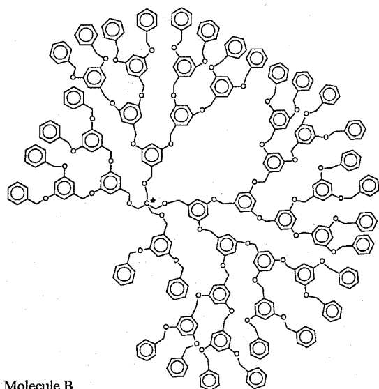
Figure 4. Chiral dendrimers A and B consisting of a chiral core to which four constitutionally different wedges are attached [23].
