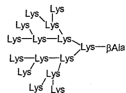
Figure 2. Tam's all-peptide dendrimer [8].
