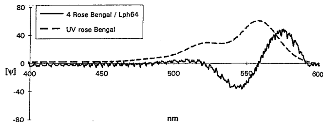
Figure 10. Induced CD effect for encapsulated Rose Bengal molecules in a dendritic box [32].
