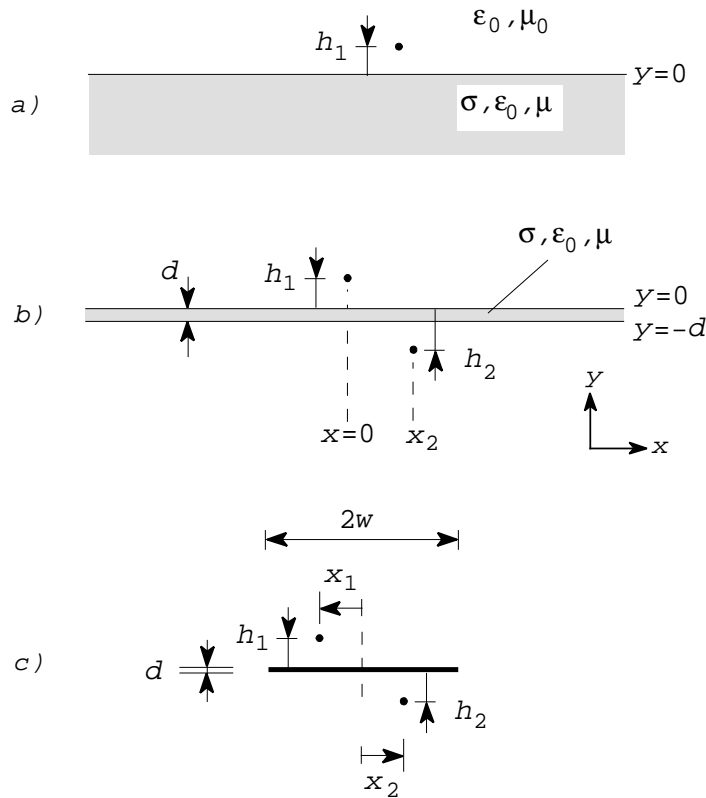
Fig. 6. Parameters for a) the infinite plane, b) the infinite plate, and c) the strip or finite plate.
