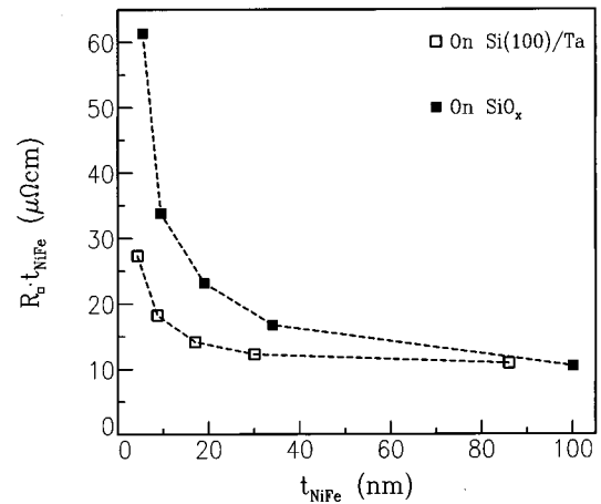
FIG. 5. The product of the sheet resistance and the \text{Ni}_{80}\text{Fe}_{20} layer thickness R_{\square} \cdot t_{\text{NiFe}} as a function of t_{\text{NiFe}} , measured at 5 K for the textured (on \text{Si}(100)/\text{Ta} ) and untextured (on \text{SiO}_x ) films. The lines are guides to the eye.
