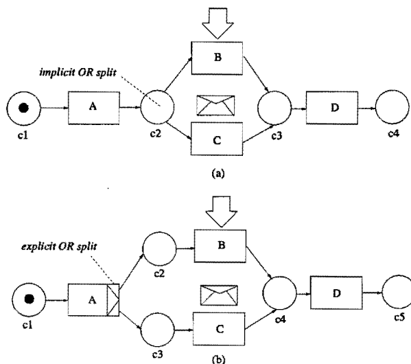
Figure 7: Illustrating the difference between implicit (a) and explicit (b) XOR-splits
