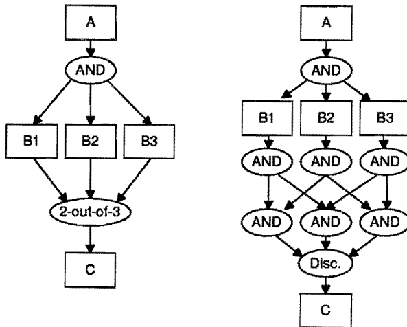
Figure 4: Implementation of 2-out-of-3-join using simple discriminator
