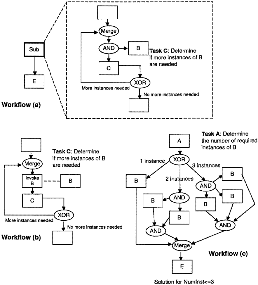
Figure 6: Design patterns for multiple instances
