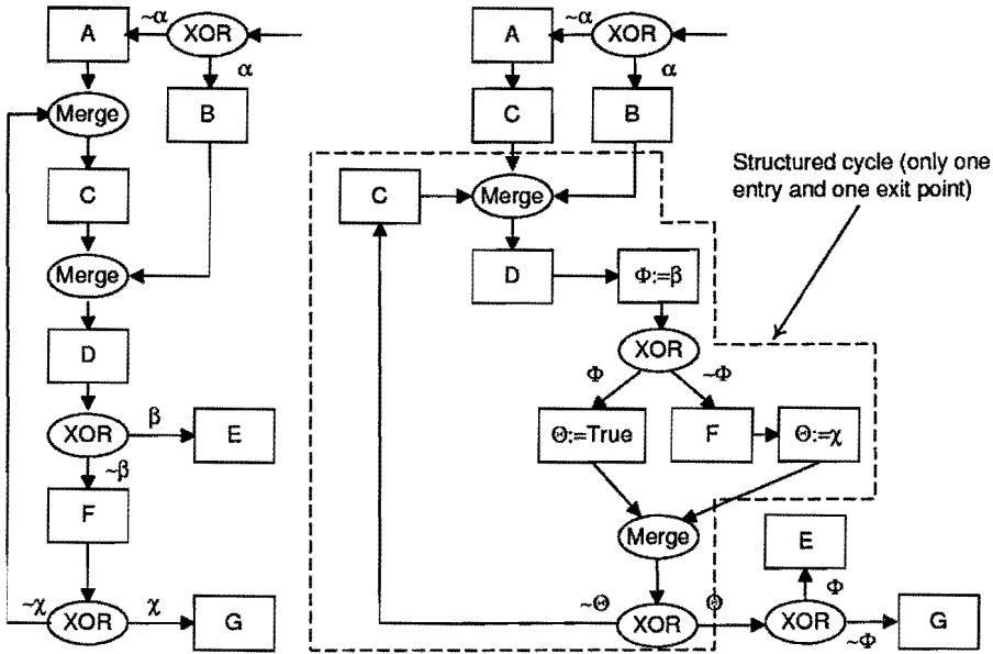
Figure 5: Implementation of arbitrary cycles
