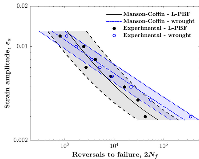
FIGURE 11 Comparison between the Manson–Coffin curves and experimental data for the L-PBF and wrought AISI 316L. The two 95% scatter bands are highlighted by transparent colors. [Colour figure can be viewed at wileyonlinelibrary.com ]
