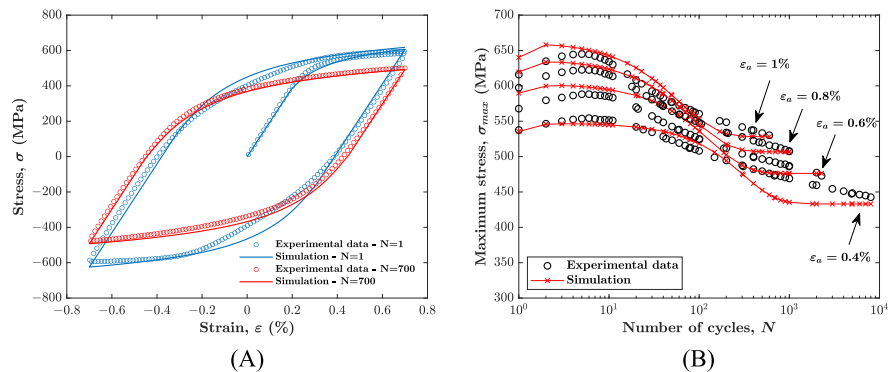
FIGURE 5 Comparison between experimental and simulated cyclic plasticity behavior: (A) 1st and 700th stress-strain cycle at \epsilon_a = 0.7\% ; (B) maximum stress versus number of cycles up to N_f/2 for four different strain amplitudes. [Colour figure can be viewed at wileyonlinelibrary.com ]
