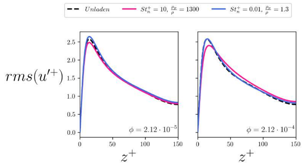
Figure 14. Root mean square (rms) of the streamwise fluid velocity along the wall-normal coordinate. The left panel refers to the \phi = 2.12 \cdot 10^{-5} case, the right panel refers to the \phi = 2.12 \cdot 10^{-4} case. The curves relative to the St_n^+ = 0.01 fibers are plotted in blue while the curves relative to the St_n^+ = 10 fibers are plotted in pink. The curve of the unladen flow case is plotted in dashed black for reference. All cases are normalized according to the shear velocity yield by the corresponding simulation.
