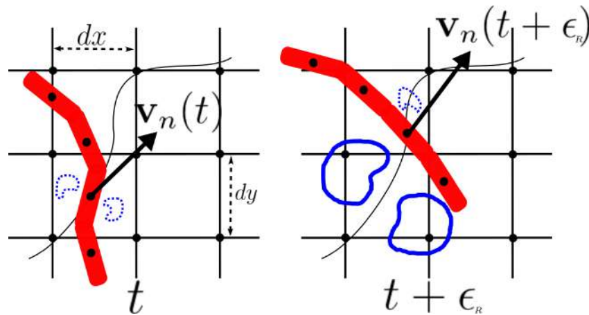
Figure 5. Schematic representation (freely inspired by [26]) of the two-way coupling according to the ERPP method. Left panel: the disturbance generated by the n th element moving with velocity \mathbf{v}_n(t) at the time-step t has yet to diffuse to the computational grid, whose spacing is indicated by dx and dy . Right panel: At time t + \epsilon_R , the n th element has moved along its trajectory while the previously generated disturbance has diffused enough to reach the computational grid with delay \epsilon_R .
