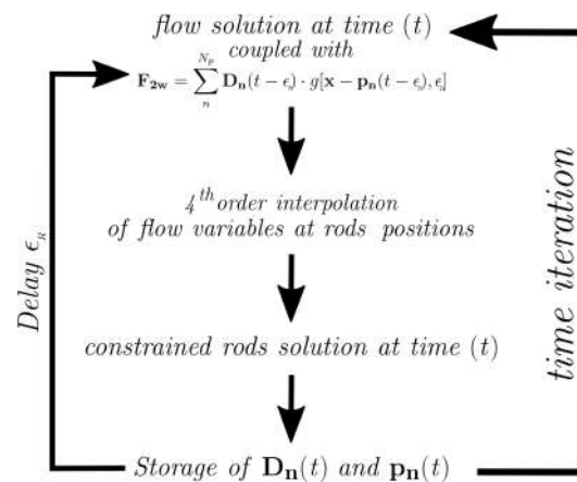
Figure 6. Schematic representation of the method of study: all the simulations performed in this study start from a random dispersion of mean-flow-aligned fibers at a given volume fraction in fully-developed turbulent channel flow. Then, the calculations are advanced in time, storing the instantaneous position of each fiber element, \mathbf{p}_n , and the drag force experienced by the element, \mathbf{D}_n over a time window whose length is given by the ratio between the delayed time scale \epsilon and the value for the time step, dt . Once one full delayed time scale has expired, the two-way coupling term \mathbf{F}_{2w} can be calculated and added as a source term in the governing equations for the fluid, 1a, b . The loop is then repeated until the end of the simulation.
