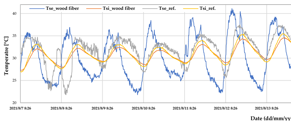
Figure 5. Trend of the internal and external surface temperature of the insulated and reference building (period between 7 and 13 August 2021).
