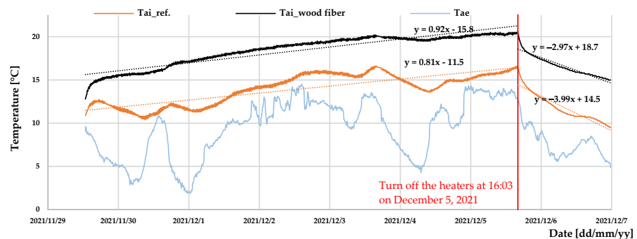
Figure 9. Trend of the air temperature of the insulated and reference building with electric fan heaters set at 600 Watts.
