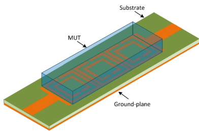
Figure 12. Setup of the TC-SRR sensor with MUT placed over the three SRR unit-cells.
