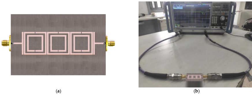
Figure 17. (a) Fabricated TC-SRR sensor. (b) Measurement setup for TC-SRR using R&S ZND Vector Network Analyzer.
