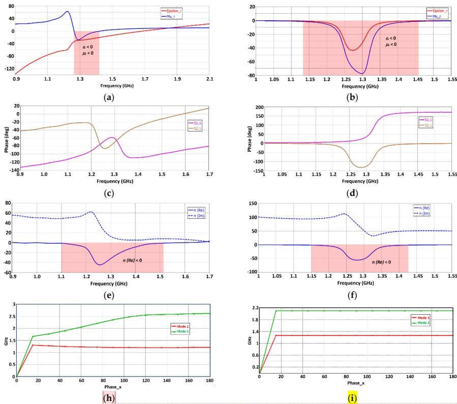
Figure 3. Characteristics of the conventional complementary split-ring resonator (SRR) and modified SRR unit-cell (M-SRR). (a) SRR; (b) Modified SRR; (c); (d) Modified SRR; (e); (f) Modified SRR; (h); (i) Modified SRR.
