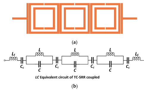
Figure 9. Sensor based on the tri-composite split-ring resonator (TC-SRR). (b) Simplified equivalent circuit model of TC-SRR.
