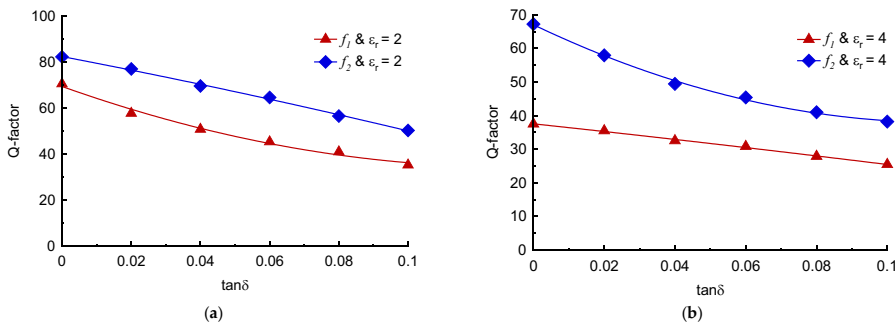
Figure 16. Q-factor versus loss tangent of TC-SRR sensor with MUT samples of permittivities ( \epsilon_r ) 2 and 4.
