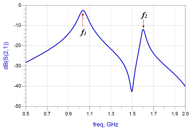
Figure 5. Transmission response of the proposed M-SRR unit-cell.
