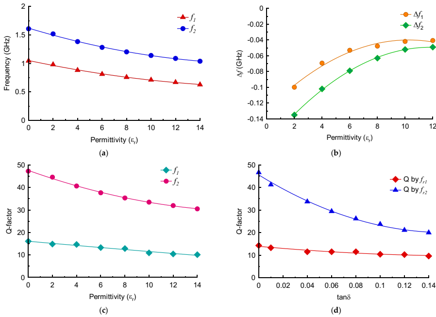
Figure 7. (a) Resonant frequency of the M-SRR sensor as a function of MUT permittivity. (b) Change in the resonant frequency of the M-SRR sensor as a function of MUT permittivity. (c) Q-factor of the two frequency responses with increase in MUT permittivity. (d) Q-factor as a function of loss tangent of the MUT.
