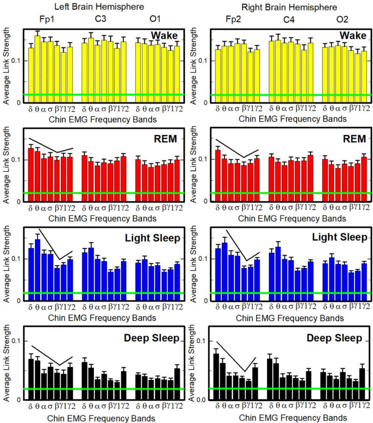
FIGURE 12 | Characteristic profiles of network links strength representing interactions between integrated brain activity at cortical areas and individual chin-EMG frequency bands. Group-averaged links strength is obtained using the TDS method (Materials and Methods section 2.3), where each link represents the interaction of brain activity from a given cortical area (averaged over all brain waves derived from the EEG channel located at this cortical area) and each muscle tone rhythm
