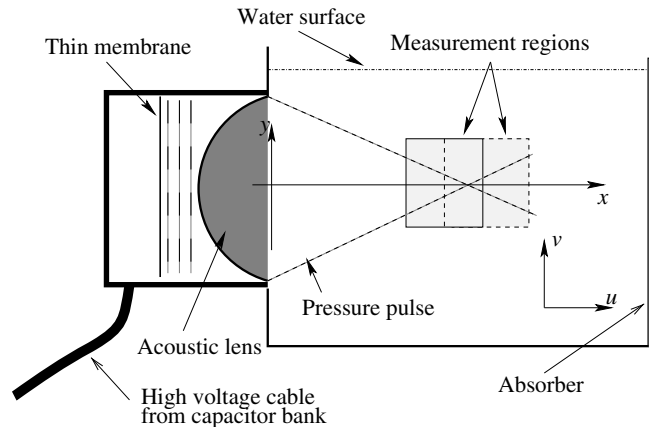
Figure 1. Schematic of lithotripter and tank arrangement.
