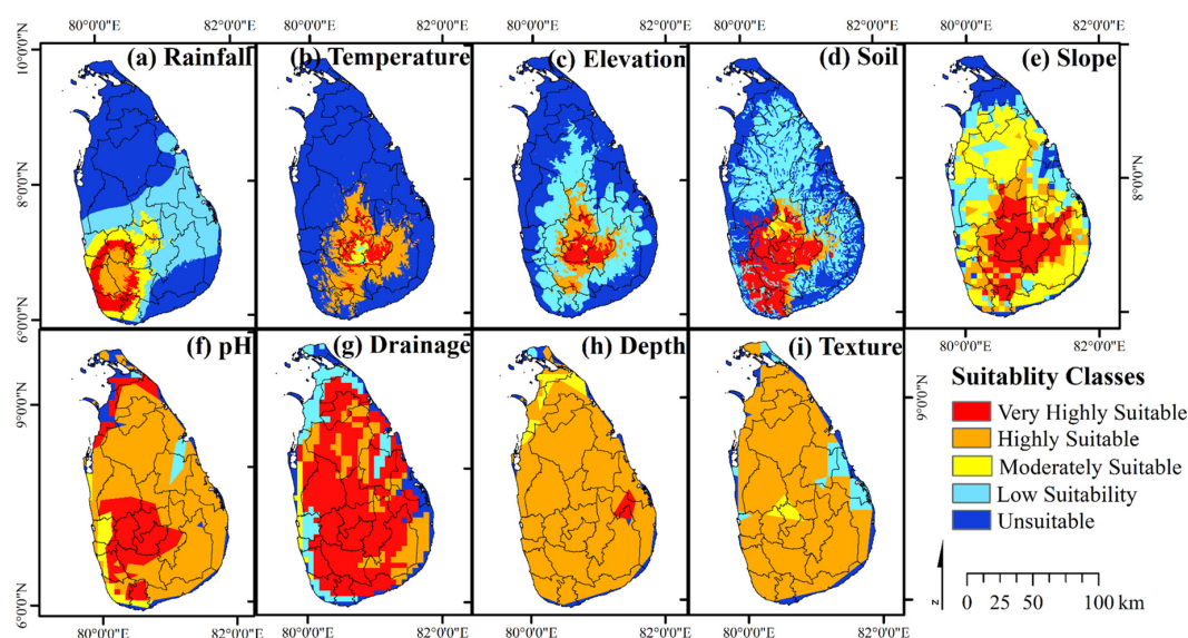
Figure 3. Criteria distribution maps of the study area climatic factors (rainfall (a) and temperature (b)), elevation (c), soil types (d), slope (e), and other soil characteristics (pH (f), drainage (g), depth (h) and texture (i)).
