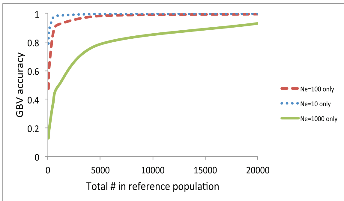
Fig 6. Accuracy of GBV when using N_e = 1000 only, N_e = 100 only and N_e = 10 only with a heritability of 0.25 ( A ), and with a heritability of 0.75 ( B ). For N_e = 10 only, the accuracy at a sample size of 100 was 0.73 ( A ) and 0.88 ( B ). For N_e = 100 only, the accuracy at a sample size of 1000 was 0.81 ( A ) and 0.92 ( B ). For N_e = 1000 only, the accuracy at a sample size of 20,000 was 0.83 ( A ) and 0.93 ( B ).
