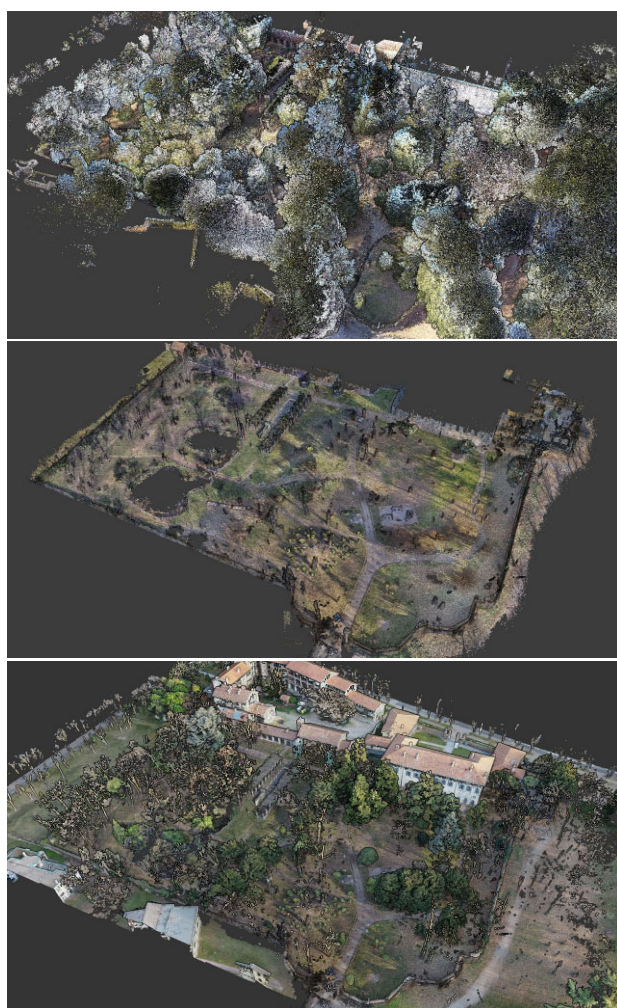
Figure 5. Point clouds obtained for the various survey carried out: Heron Backpack (top), Ant3D (centre), UAV (bottom).
