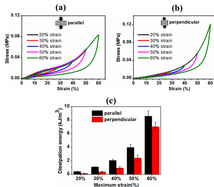
Figure 10. Compressive mechanical properties of the Gel-PEG hybrid hydrogel at different maximum strains: (a) the hysteresis loops when compressed in parallel and (b) perpendicular to the macroporous channels at different maximum strains and (c) corresponding hysteresis energies of the hydrogel compressed in parallel and perpendicular directions.
