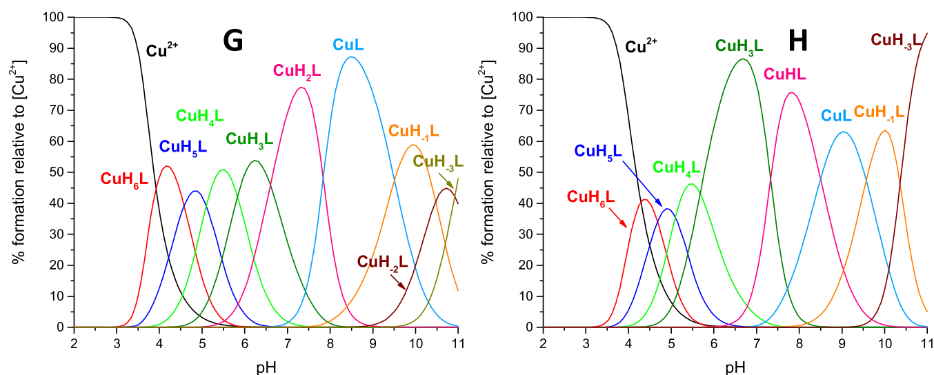
Figure 2. Distribution diagram of complex forms in the Cu(II)-L systems. L—Ac-DHDHHHGHAAH (A), Ac-DKPAKAEDDHHHGHAAH (B), Ac-DKPAKAEDQDHHHGHAAH (C), Ac-DKPAKAEDHDQHHHGHAAH (D), Ac-DKPAKAEDHDHQHHHGHAAH (E), Ac-DKPAKAEDDHHHGHAAH (F), Ac-DKPAKAEDDHHHGQAAH (G), and Ac-DKPAKAEDDHHHGHAAQ (H). M/L = 1:1. pH range: 2–11.
