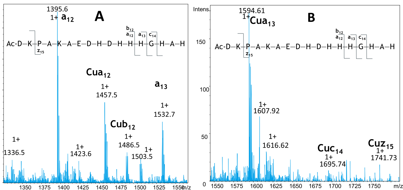
Figure 5. ESI-MS/MS spectrum of the Cu(II)-L2 sample at (A) 1325–1575 m/z range and (B) 1550–1775 m/z range. Parent ion m/z = 1021.93 , z = 2+ ; collision energy 40 eV. The fragmentation pattern was assigned. 41
