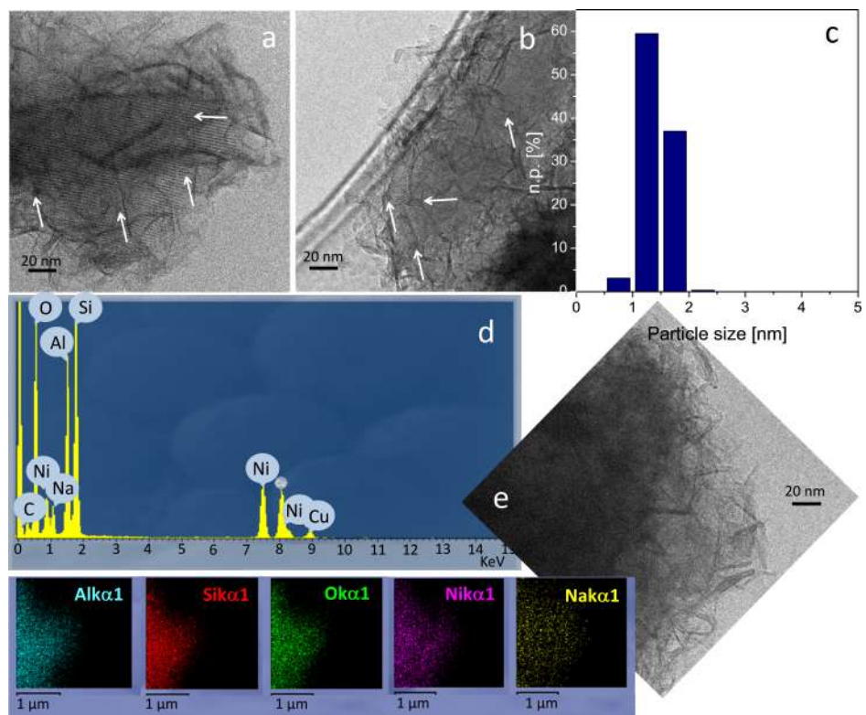
Figure 5: Representative HRTEM (a and b) and TEM (e) images of the \text{Ni}^{2+} _X sample and Ni-containing particle size distribution (c). EDS spectrum collected on the region shown in panel b (d). EDS maps of the region shown in panel e (f). The Ni-containing nanoparticles are highlighted by with arrows. Instrumental magnification: 100000 \times .
