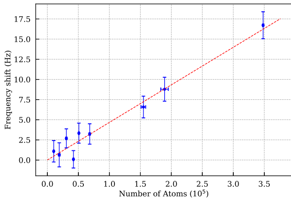
Fig. 8. Evaluation of the density shift of the ^{88}\text{Sr} clock transition. We assume linear scaling of density with atom number.
