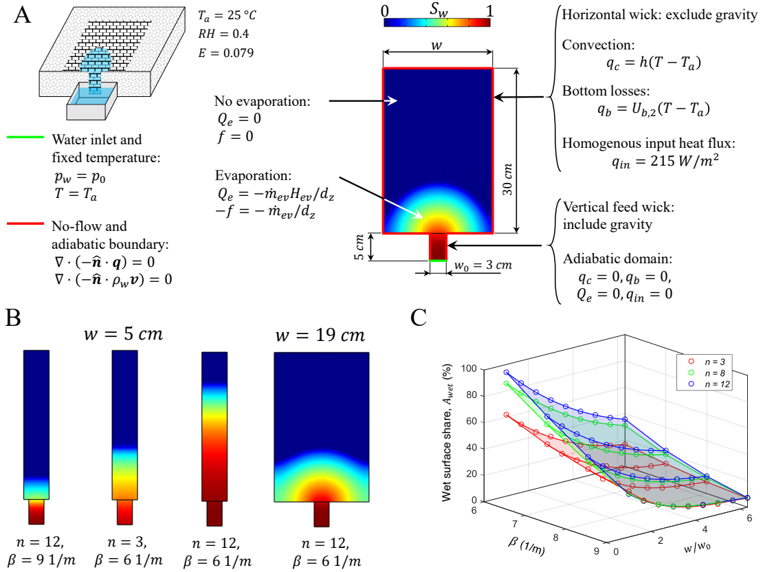
Figure 9: Design-oriented sensitivity analysis of a hydrophilic fabric for passive thermal desalination. (A) Schematics of the simulation setup and the employed boundary conditions. The setup represents a typical porous hydrophilic component of passive devices for water desalination. The component is used to adsorb salt-water from a reservoir, and feed a distillation device (or directly evaporate it) under solar light. (B) Steady states ( t = 15 \cdot 10^3 s, see Supplementary Video 2) obtained varying the values of the van Genuchten's parameters or the width of the component w . Reducing \beta and increasing n results in a higher share of wet surface A_{wet} , thus to higher efficiency of the component. (C) Sensitivity analysis to assess the relationship between the van Genuchten's parameters \beta and n , the aspect ratio of the component w/w_0 and the share of wet surface A_{wet} . Note that the simulations were performed considering distilled water.
