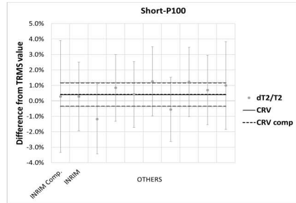
Fig. 6. T_2 's comparison and reanalysis data.
