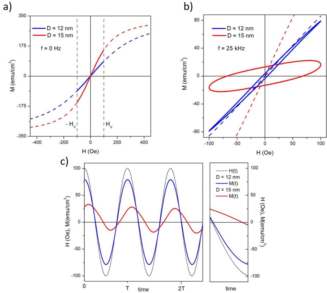
Figure 1: (a): Full lines: anhyseretic magnetization of two monodisperse nanoparticle assemblies in quasi-static conditions for H \leq H_V = 100 \text{ Oe} ; dashed lines: Langevin curves; (b): magnetic hysteresis in the same systems under a high-frequency driving field of vertex H_V ; dashed lines: Langevin curves; (c): H(t) (thin black line) and M(t) waveforms (thick lines in colour) at 25 \text{ kOe} . The phase shifts of M(t) are shown in the rightmost bottom panel.
