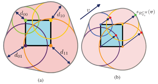
Figure 5: (a) Construction of R^{CH} in 2D. (b) Support point computation of R^{CH} in direction v . The support points of the eight spheres are computed, and any of the furthest along v is returned.
