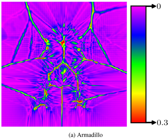
Figure 16: OpenVDB distance field algorithm absolute error. The selected slice is the same as the one used on Figure 14. The error is expressed with respect to the voxel size.
