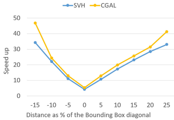
Figure 15: Speedup achieved by our method with respect to others (SVH and CGAL BVH) at different distances from the input mesh (Frog in this case).
