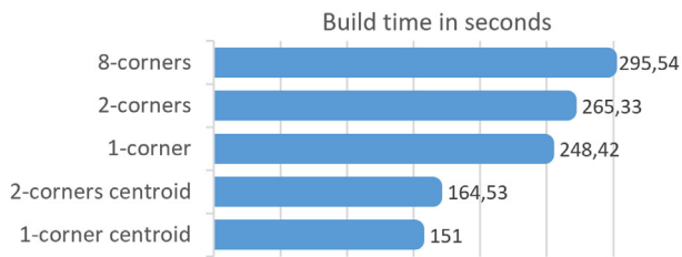
Figure 10: Octree build times with different triangle filtering strategies. Only the triangles closest to n of the eight corners of a node are used. In the options marked as centroid, distances to triangles are computed to centroids.
