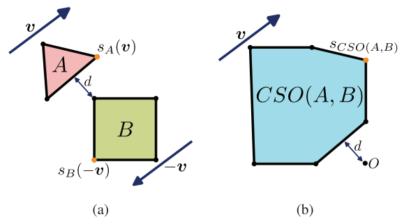
Figure 3: Example showing the Minkowski difference between two polygons, A and B . d is the minimum distance between the two polygons.
