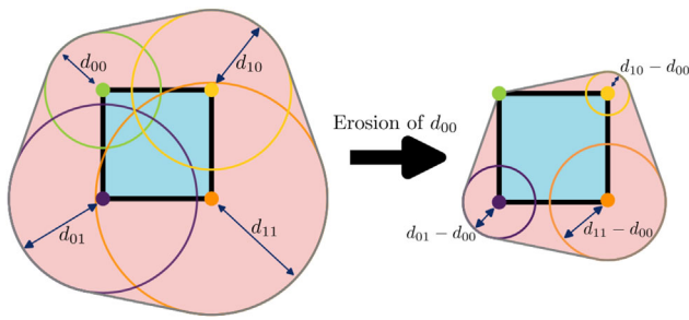
Figure 7: R_{T_c}^{CH} spherically eroded by the minimum sphere radius ( d_{00} ) to obtain \ominus R_{T_c}^{CH} .
