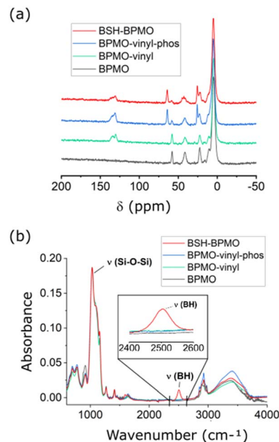
Fig. 4 Chemical characterization of BPMO nanoparticles: (a) 13 C solid-state NMR spectra of BPMO at different synthetic steps; (b) FTIR spectra. Note: The 13 C NMR signal around 57 ppm arises from the residual ethoxy group.
