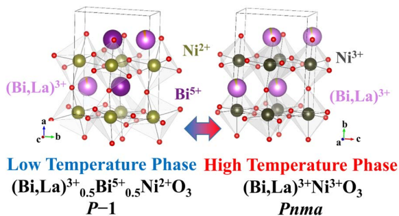
Fig. 1 Schematic illustration of the intersite charge-transfer transition in \text{Bi}_{0.95}\text{Ln}_{0.05}\text{NiO}_3 . The high-temperature Pnma (\text{Bi,La})^{3+}\text{Ni}^{3+}\text{O}_3 phase changes to the low-temperature P-1 (\text{Bi,La})^{3+}_{0.5}\text{Bi}^{5+}_{0.5}\text{Ni}^{2+}\text{O}_3 phase by intersite charge transfer between Bi and Ni ions.
