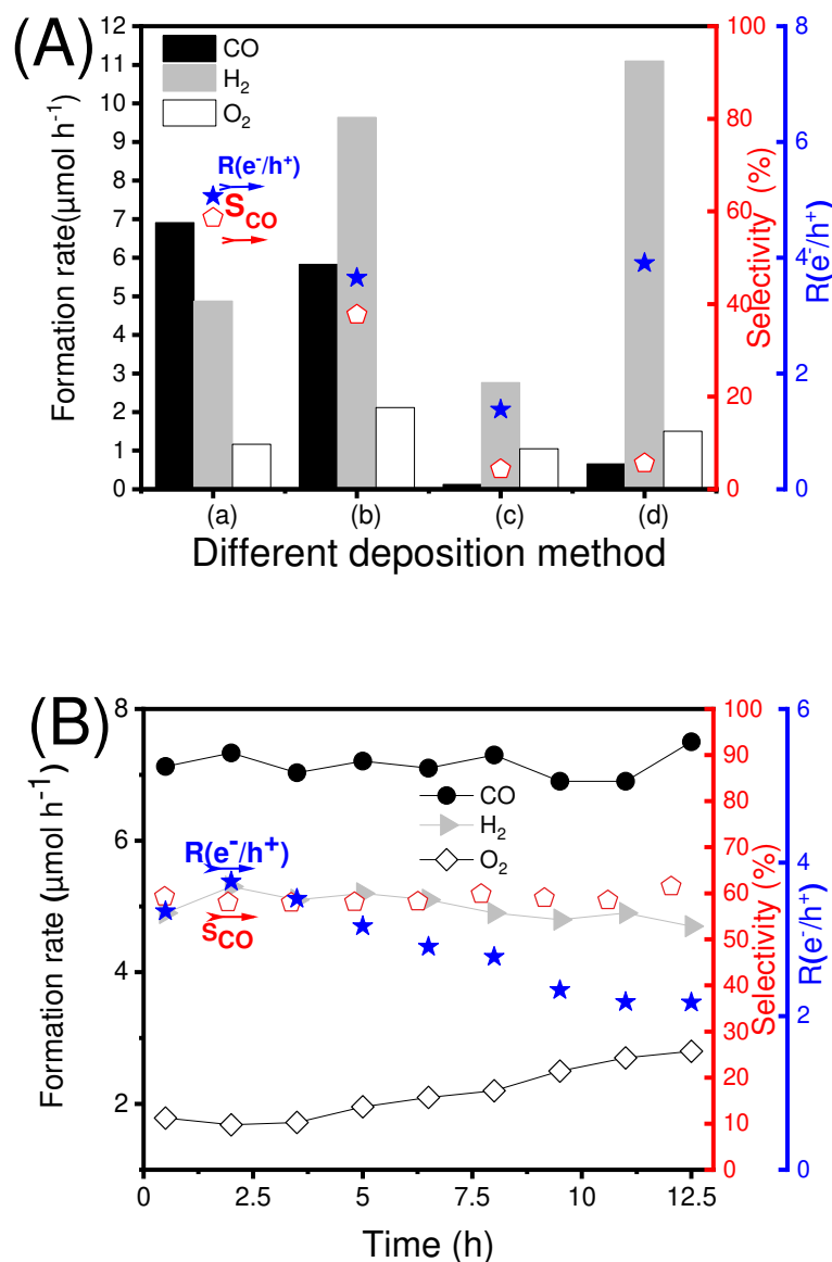
Fig. 5. [A] Formation rates of CO, H 2 , and O 2 , the CO selectivity in the reductive products ( S_{CO} ), and the electron and hole ratio consumed for the gaseous product formation R(e^-/h^+) , in the photocatalytic reaction test for CO 2 conversion in the aqueous solution over the photocatalyst samples; (a) Ag(PD)-NiO x (PD)/CTO, (b) Ag(PD)/NiO x (IMP)/CTO, (c) Ag(IMP)-NiO x (IMP)/CTO, and (d) NiO x (IMP)/Ag(PD)/CTO. The data were taken after the photoirradiation for 4.5 h. [B] Time course of the production rates in the gas phase, S_{CO} , and R(e^-/h^+) in the photocatalytic reaction test for CO 2 conversion in the aqueous solution with the Ag(PD)-NiO x (PD)/CTO sample.
