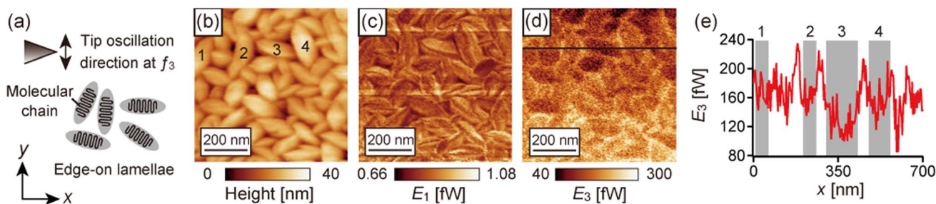
Fig. 10 The bimodal AFM results on the P(VDF-TrFE) film obtained at 125 °C under ambient conditions. (a) Schematic illustration of the P(VDF-TrFE) edge-on lamellae and tip oscillation at f_3 . (b) Topography. (c) Energy dissipation in the first mode E_1 . (d) Energy dissipation in the third mode E_3 . (e) Line profile of E_3 on the black line in (d). The gray-colored zones in (e) correspond to the numbered grains indicated in (b). The probe length l and the etched part length l_c were 1.61 mm and 0.17 mm, respectively. f_1 = 11.6 kHz, Q_1 = 1600 , k_{1,v} = 1.9 kN m ^{-1} , \theta_1 = 41.7^\circ , A_1 = 118 pm, f_3 = 142.6 kHz, Q_3 = 550 , k_{3,l} = 58.6 kN m ^{-1} , \theta_3 = 6.3^\circ , and A_{3,0} = 386 pm. Q_1 and Q_3 are the quality factors of the first and third modes, respectively. A_{3,0} is the free amplitude of the third mode. These images were taken at \Delta f_1 = +3.5 Hz.
