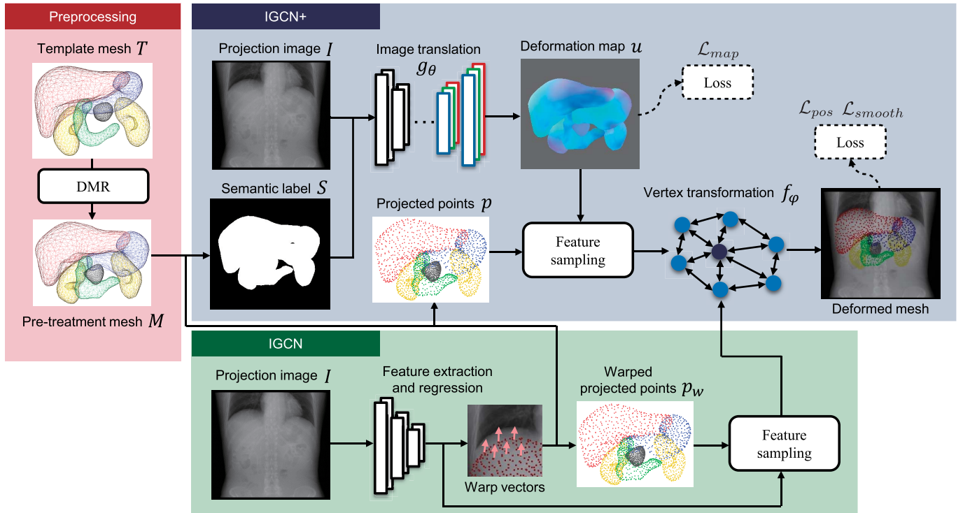
Fig. 2. Full IGCN+. The image translation network g_\theta learns to generate a displacement field u . The vertex coordinates and corresponding 3D displacement vectors are concatenated into the GCN f_\phi for mesh deformation learning. IGCN relies on both feature extraction and reference point optimization in the CNNs.
