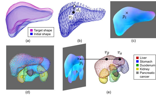
Fig. 3. Learning scheme for image translation function generating spatial mapping function u . (a) DMR between initial and target 3D shapes, (b) 3D displacement vectors obtained from corresponding vertices, (c) forward displacement map and sampling, (d) displacement map in abdominal regions overlaid with their meshes, and (e) one-to-many correspondence between displacement field and mesh.
