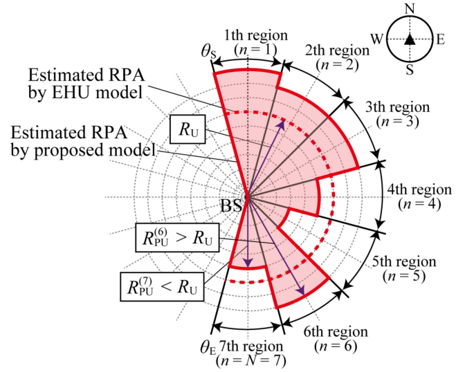
FIGURE 10. Example of RPA estimated using the proposed model in an urban area.
