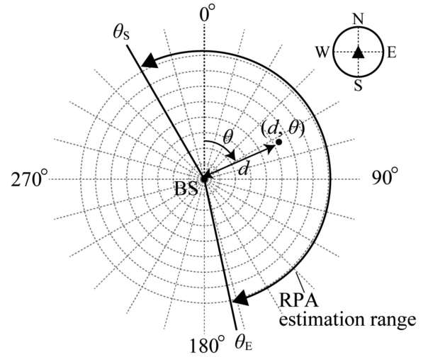
FIGURE 9. Counterclockwise polar coordinate system for RPA estimation.
