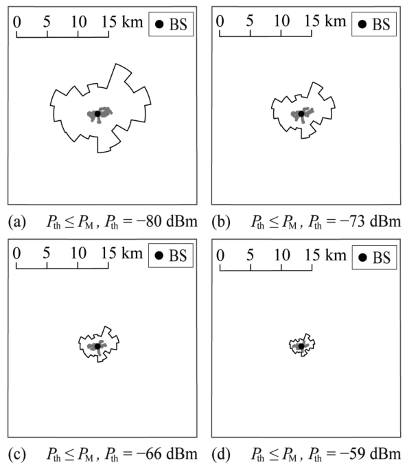
FIGURE 19. RPA estimated by the proposed model with Method-B in a suburban area.
