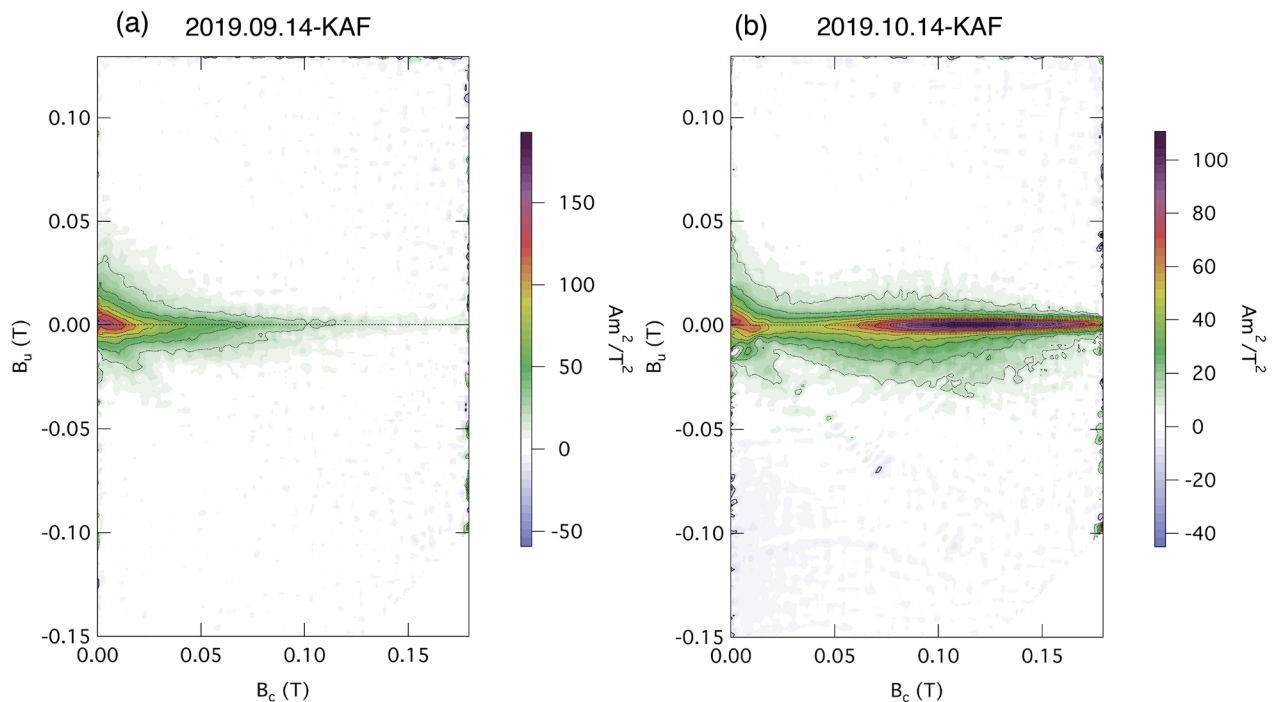
Fig. 3 Results of FORC measurement. a FORC diagram for the sample of September 14, 2019, collected from the KAF station. b FORC diagram for the sample of October 14, 2019, collected from the KAF station. Ash samples from October 14 indicate the presence of non-interacting SD grains with high coercivity and a narrow range of B_u values
