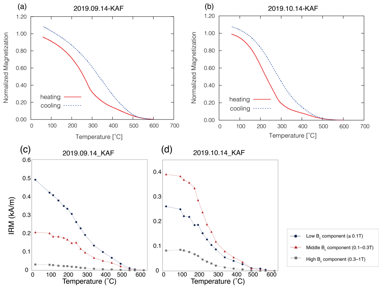
Fig. 1 Results of thermomagnetic analyses and thermal demagnetizations of a 3-axis composite IRM. a Thermomagnetic analysis in air for the sample of September 14, 2019. The red solid line is the heating curve and the blue dashed line is the cooling curve. b Result of thermomagnetic analyses in air for the sample of October 14, 2019. Legend is the same as a . c Result of thermal demagnetization of a 3-axis composite IRM for the sample of September 14, 2019. Coercivity components of \leq 0.1 T, 0.1–0.3 T, and 0.3–1 T are shown by circles, triangles, and squares, respectively. d Result of thermal demagnetization of a 3-axis composite IRM for the sample of October 14, 2019
