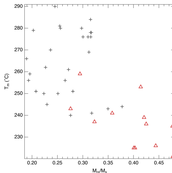
Fig. 5 T_m vs. M_{rs}/M_s of the ash samples. The HOND and KAF samples from June 6, 2020, in which no Ti-rich titanomagnetite was identified, were removed. Red triangles denote volcanic ash results when volcanic glow event was observed and gray crosses indicate those collected otherwise
