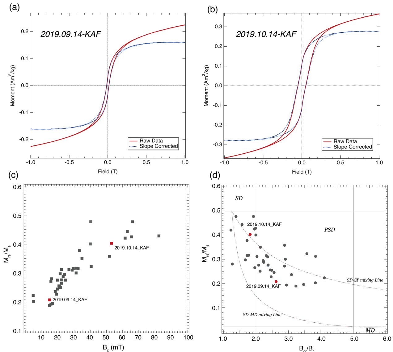
Fig. 2 Results of hysteresis measurement. a, b Examples of hysteresis loops. The red solid line is the measured hysteresis loop (raw data). The blue dashed line is the corrected loop for the effect of paramagnetic minerals. c Ratio of the saturation remanent magnetization to saturation magnetization ( M_r/M_s ) vs. coercivity ( B_c ). d M_r/M_s vs. coercivity of remanence to coercivity ( B_{cr}/B_c ). The upper left in the plot is single-domain (SD) region, while the lower right is closer to the multi-domain (MD) grain size. The two dotted lines are the SD–superparamagnetic (SP) mixing line (top) and the MD–SD mixing line (bottom) (Dunlop 2002a, b)
