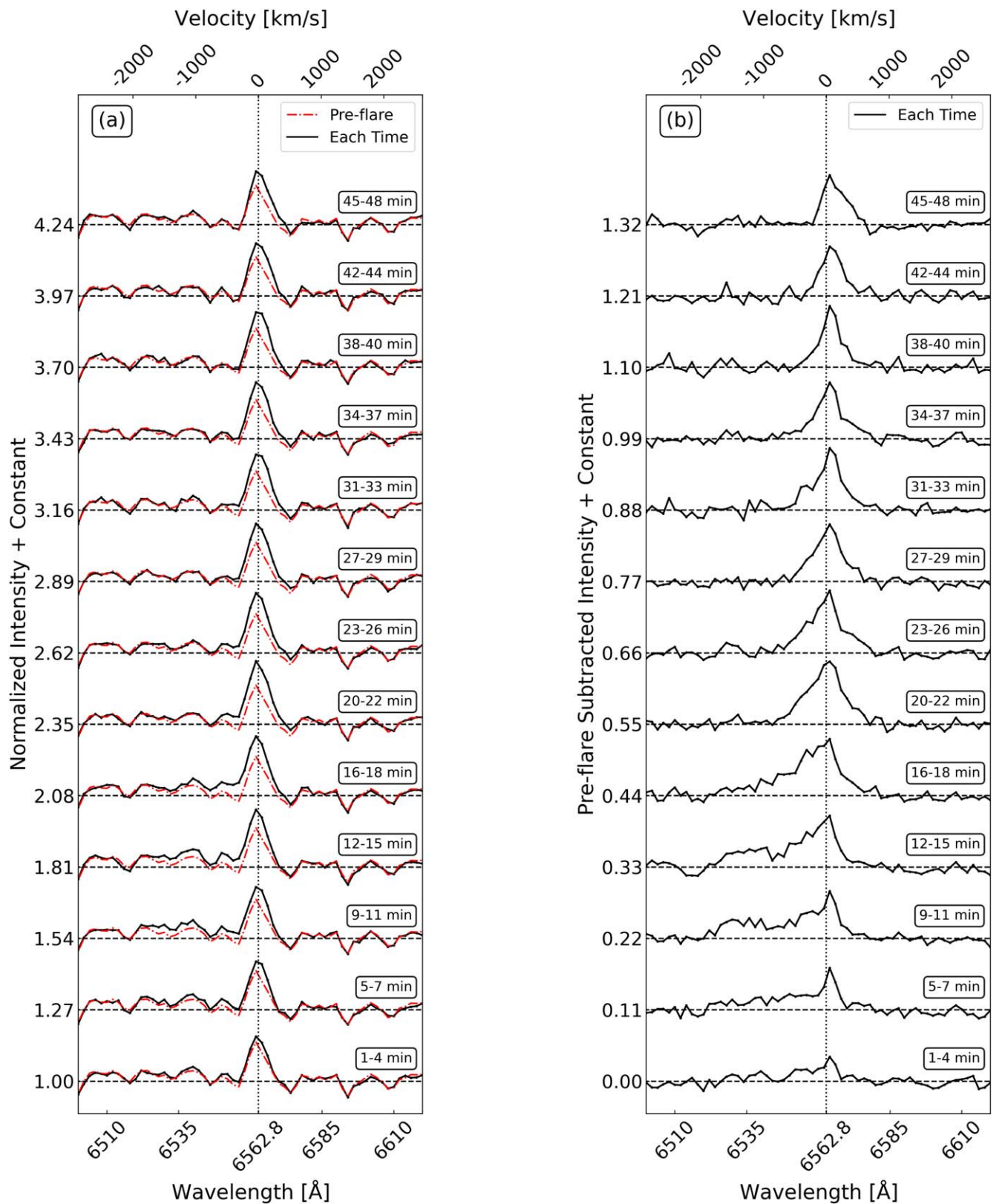
Figure 3. Time variation of the H \alpha spectrum in the early stages of the flare. (a) Line profile of H \alpha emission. Each spectrum is a composite of three (= 3 minutes) spectra. The bottom and top axes are the wavelength and Doppler velocity from the line center, respectively. The intensity of each spectrum is normalized by the continuum. The vertical dotted and horizontal dashed lines represent the line center of H \alpha and the continuum level for each spectrum, respectively. The spectrum at each time is vertically shifted, and the time shown in the upper right corner of each spectrum represents the time from the flare start. The red dashed-dotted lines represent the spectra at the pre-flare (-15 minutes to 0 minutes). (b) Pre-flare subtracted spectrum displayed in the same manner as in panel (a). The horizontal dashed line represents the zero level for each spectrum. The black minus red in panel (a) denotes the spectrum at each time.
