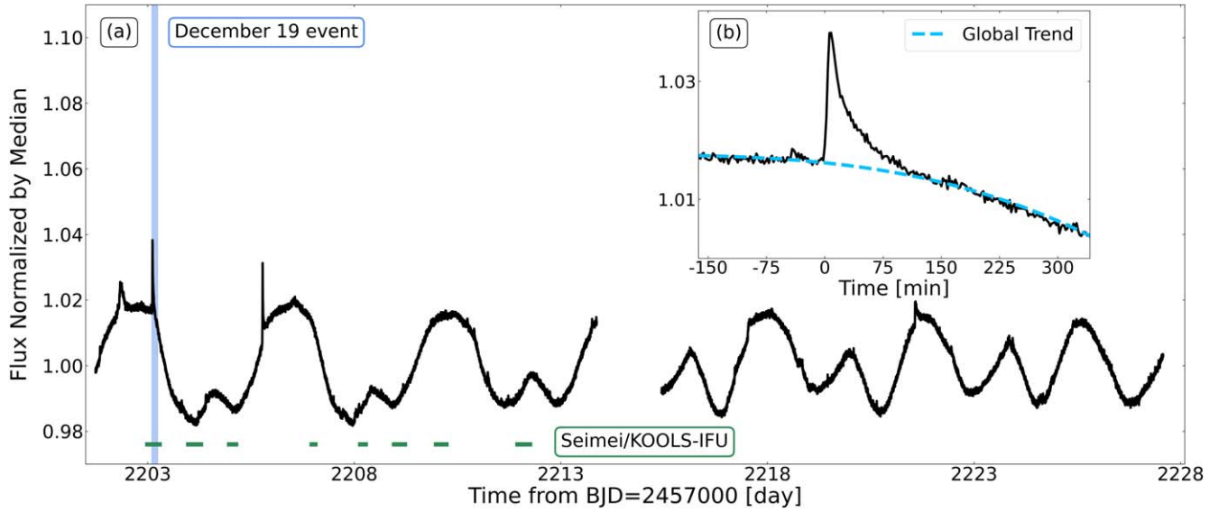
Figure 1. White-light light curves of V1355 Orionis observed with TESS. (a) Long-term light curve of V1355 Orionis for BJD = 2459201.7–2459227.5. The vertical axis represents the flux normalized by the median value. The vertical light-blue line and the horizontal green bars indicate the event discussed in this paper and the period of monitoring observations by Seimei telescope/KOOLS-IFU, respectively. (b) Enlarged light curve around December 19/BJD = 2459203.11297. The horizontal axis represents the time (unit of minutes) from BJD = 2459203.11297. The sky-blue dashed line shows the global trend of the stellar rotational modulation fitted for -500 – 10 minutes and 150 – 380 minutes with a polynomial equation.
