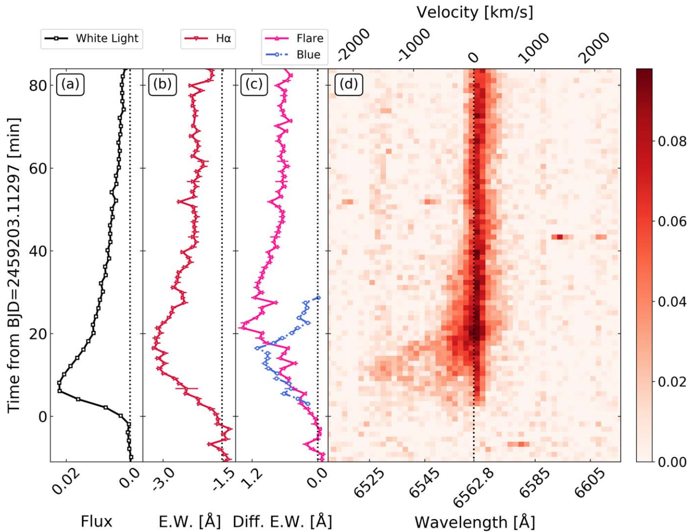
Figure 4. Light curves and spectra during a superflare on V1355 Orions. (a) Enlarged early part of the light curve of Figure 2(a). The horizontal and vertical axes indicate the detrended flux and time (unit of minutes) from BJD = 2459203.11297, respectively. (b) Enlarged H \alpha light curve of Figure 2(b) for the same period as in panel (a). The horizontal and vertical axes represent the equivalent width of H \alpha and the same vertical axis as in panel (a), respectively. (c) H \alpha light curve divided into line center and blueshifted excess components. The pink triangles and blue circles indicate the equivalent widths of the flare and blueshifted excess components, respectively. The equivalent width of the flare component was calculated by integrating the differential spectrum from the pre-flare level \pm 17 \text{\AA} from the H \alpha line center while the blueshifted excess component was not present. For the time period when the emission line was blueshifted, the equivalent width was calculated by integrating the Voigt function that fits the spectrum at longer wavelengths than the peak (e.g., the black dotted line in Figure 5(a)). The equivalent width of the blueshifted excess component was calculated by integrating the residuals between the spectra and the fitted Voigt functions (e.g., the blue line in Figure 5(b)). See Section 4.1 for more information about fitting. (d) Time variation of the differential spectrum from the pre-flare level at the same time as in panels (a), (b), and (c). The bottom and top abscissas are the wavelength and Doppler velocity from the line center, respectively.
