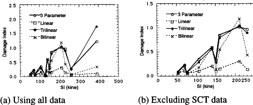
Fig. 11 Relation of damage index to the maximum velocity of input motions.
