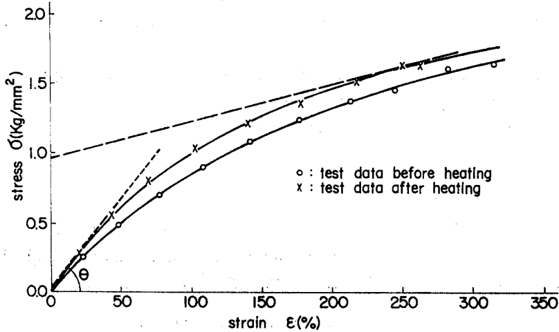
Fig. 3 Stress-strain relation
