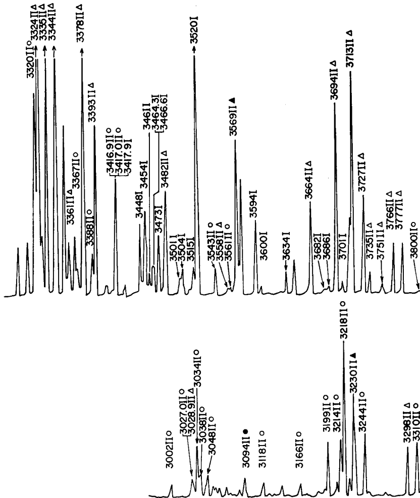
Fig. 11. The spectrum of the neon plasma produced by the electron beam, 5 mm downstream from the accelerating electrode. p=1 torr. I: NeI and II: NeII. \circ : 3p-3d , \bullet : 3p-4r , \triangle : 3s-3p and \blacktriangle : 3s'-3p' .
