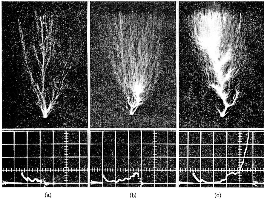
Fig. 12. Development of leader: \rho=2 mm, \delta=15 cm, chopped voltage, rod positive, V_p=117 kV, current: 2.96 A/div., 0.5 \mu\text{s/div.}
