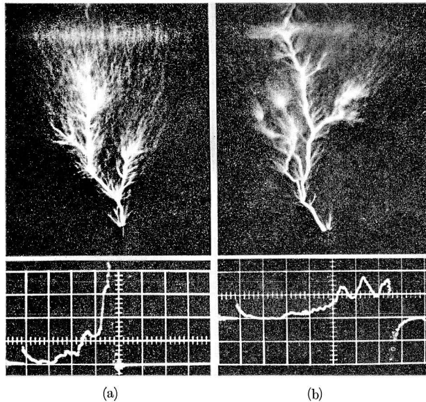
Fig. 19. Effect of insulator thickness for leader development. \rho=2 mm, \delta=10 cm, rod positive, V_p=89.7 kV. Chopped voltage. current: 2.96 A/div., 0.5 \mu s/div. (a) insulator thickness 0.8 mm, T_c=2.4 \mu s (b) insulator thickness 3 mm, T_c=3.8 \mu s
