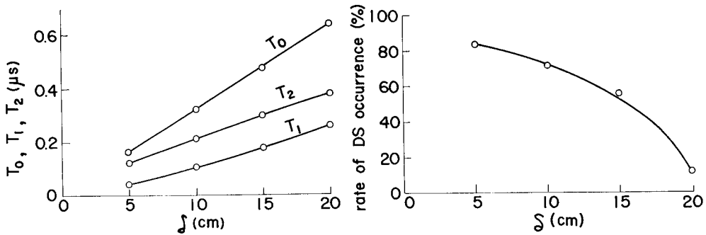
Fig. 5. T_0, T_1, T_2 vs. \delta at 50% FO voltage. \rho = 2 mm, rod positive.
