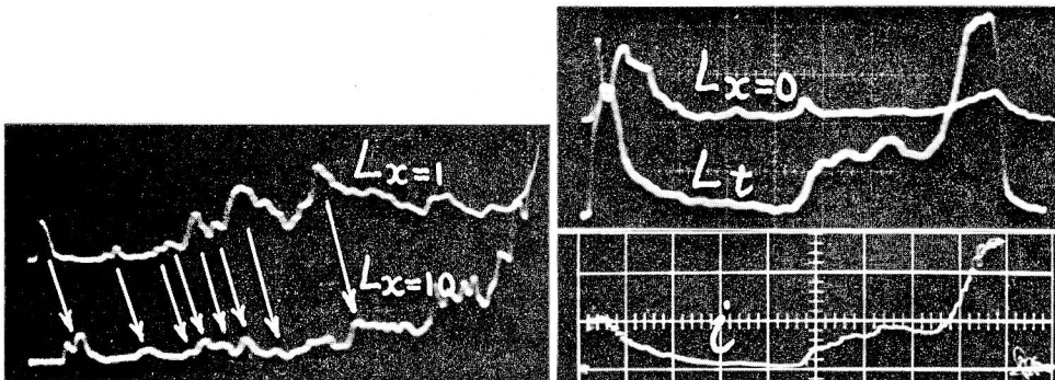
Fig. 13. Shift of light pulses for leader development: \rho=2 mm, \delta=10 cm, rod positive, V_p=89.7 kV. upper trace: x=1 cm, Lower trace: x=10 cm, sweep: 0.2 \mu\text{s/div.}
