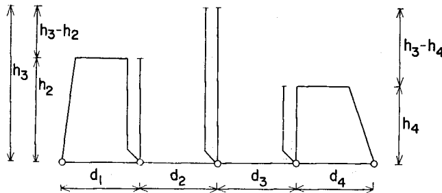
Fig. 13. Initial State of Sequential File Method for Tree System with Three Centres
