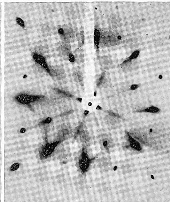
Photo. 26. Al-4.00% Cu alloy W. Q. and aged 1 day at 110°C.
