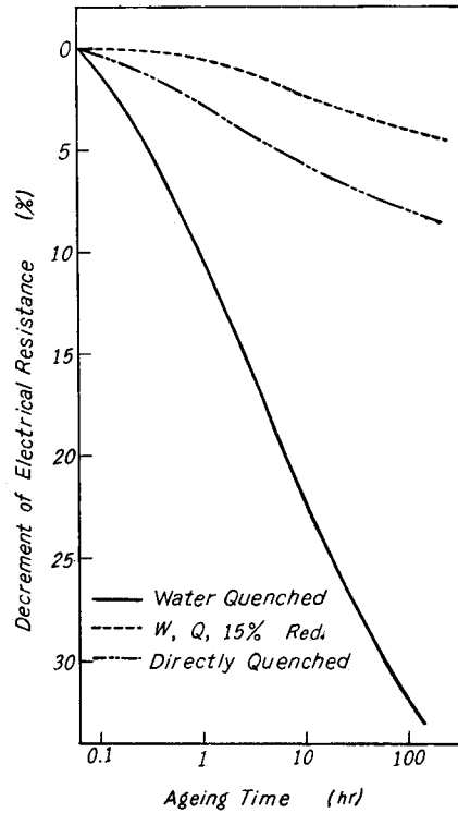
Fig. 12. Effect of direct quenching on the electrical resistance change of Cu-Ti alloys in isothermal ageing at 250°C.
