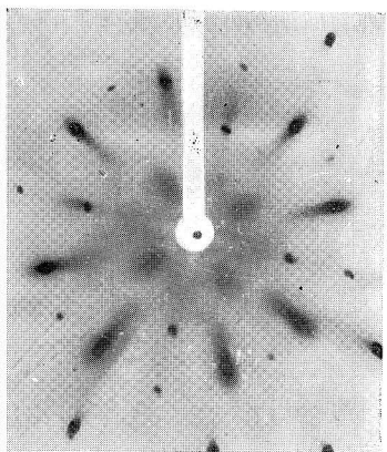
Photo. 3. Specimen shown in Photo. 1, aged 20 days at 110°C.
