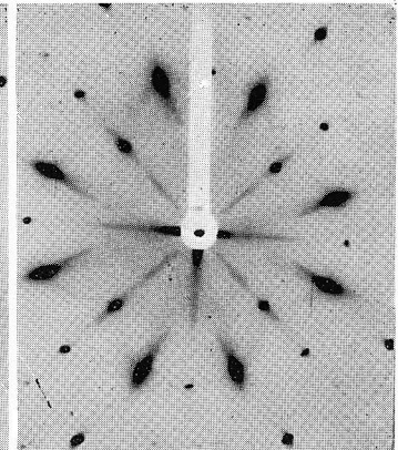
Photo. 27. Al-4.00% Cu alloy W. Q., elong. 7.5% and aged 1 day at 110°C.
