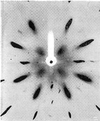
Photo. 4. Specimen shown in Photo. 2, aged 20 days at 110°C.
