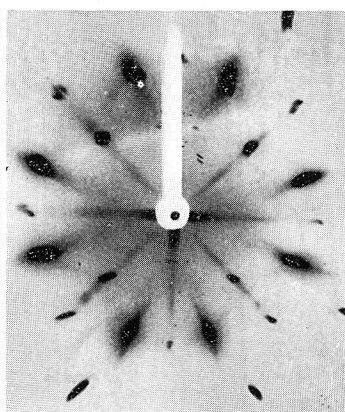
Photo. 41. Specimen shown in Photo. 35, aged 1 day at 110°C.
