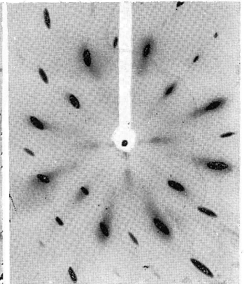
Photo. 9. Specimen shown in Photo. 6, aged 22 days at 70°C.
