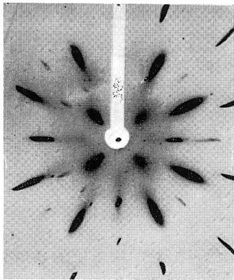
Photo. 2. Al-16.51% Ag alloy W. Q. and elongated 5.3%.
