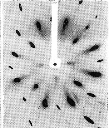
Photo. 6. Al-1.80% Cu alloy W. Q. and elongated 6.3%.
