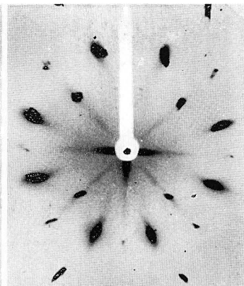
Photo. 39. Specimen shown in Photo. 35, aged 5 hr at 110°C.
