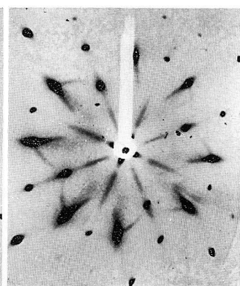
Photo. 42. Specimen shown in Photo. 34, aged 3 days at 110°C.
