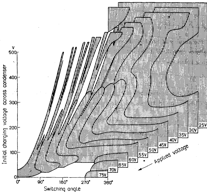
Fig. 6. Regions of initial conditions for the resonant oscillation (blank) and for the non-resonant oscillation (shaded) obtained under several values of the applied voltage.
