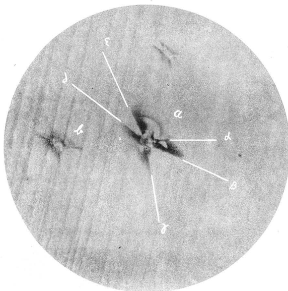
Fig. 1. Tear-figures on (111) of copper-sulphate crystal. a.....a perfect form with cracks parallel to \{100\} , \{\bar{1}\bar{1}0\} and \{010\} . b.....an imperfect one with a rhombic body, whose sides are parallel to \{110\} and \{\bar{1}\bar{1}0\} and four rays, two of which are parallel to \{100\} and \{\bar{1}\bar{1}0\} . The parallel streaks through the photomicrograph are polishing scratches. Transmitted light. Mag. 115 diam.
