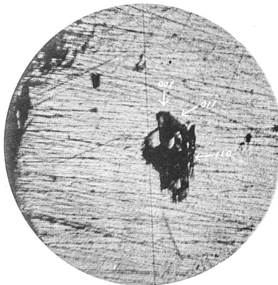
Fig. 2. Tear-figure on the (100) face of enargite. The six-sided type bounded by sides parallel to (00\bar{1}) , (01\bar{1}) , (1\bar{1}0) , (0\bar{1}\bar{1}) (00\bar{1}) , and (1\bar{1}0) . The rounded image on the left hand is the pit of a pin's point. The direction of the vertical axis from North to south. Vert. illum. Mag. 60 dia.
