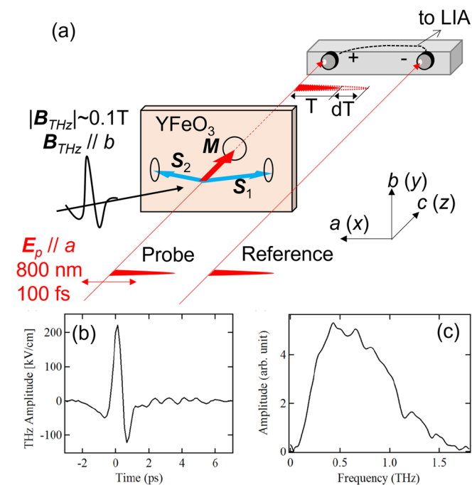
Fig. 1 Schematic of the intense THz pump-induced magnetorefractive measurement. a Experimental setup. The blue and red arrows indicate the sublattice magnetizations S_{1,2} and net magnetization M , respectively. RT Room temperature, BPD Balanced photodetector, LIA lock-in amplifier. b Typical waveform of the THz electric field measured with electrooptic sampling in a GaP (110) single crystal with 400 \mu\text{m} thickness. c Fourier spectrum of b .
