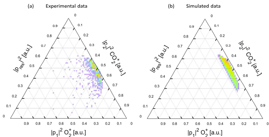
Figure. 5.17 The experimental and simulated Region B of the momentum correlation of the O_2^+/CO_2^+ ion pair produced from CO_2 clusters with cluster size N_{\text{mean}} \sim 20 . (a) shows the filtered experimental momentum correlation of the O_2^+/CO_2^+ ion pair to extract only the Region B of the Dalitz plot. (b) shows the simulated data using the intracluster collision model described in the text using the chemical reactions in (5.2.26) and (5.2.27).
