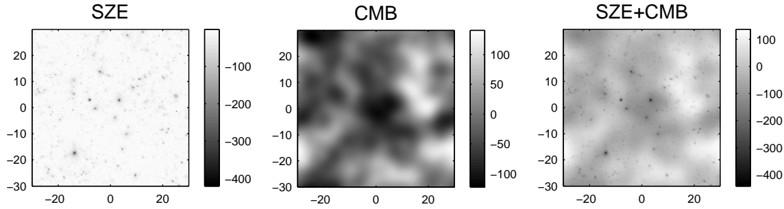
Figure 2.8. Illustration of the characteristic angular scales of primary CMB anisotropy and of the SZ (Carlstrom et al., 2002). The images each cover one square degree and the grey scales are in \mu\text{K} . The left panel shows a image of the SZ from many clusters at 150 GHz (2 mm) obtained from a hydrodynamic simulation. The clusters appear point-like at this angular scale. The centre panel is a realization of CMB anisotropy for a \Lambda\text{CDM} cosmology. The right panel illustrates that the SZ can be distinguished readily from primary CMB anisotropy provided the observations have sufficient angular resolution.
