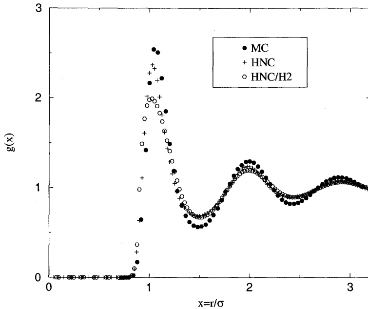
FIGURE 5.4: Comparison of the Monte Carlo (MC), the HNC, and HNC/H2 results for the pair distribution function of the inverse 6th-power fluid at z = 1.54 .
