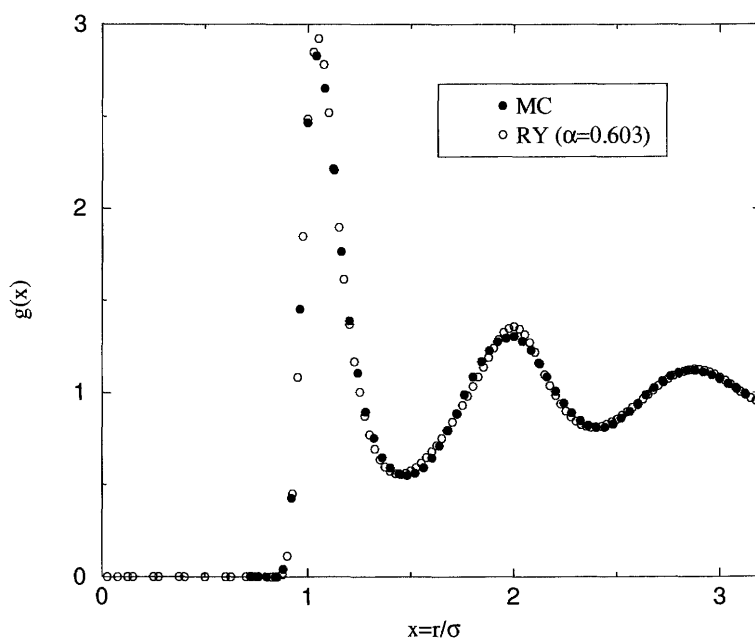
FIGURE 5.1: Comparison of the Monte Carlo (MC) and Rogers Young (RY) results for the pair distribution function of the inverse 12th-power fluid at z = 0.813 .
