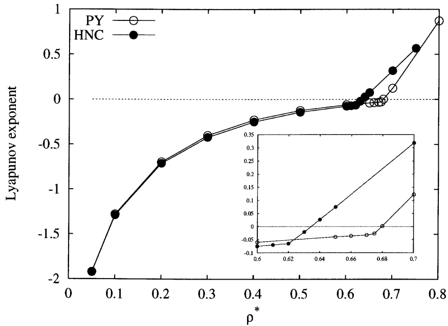
FIGURE 6.3: We show the Lyapunov exponent as a function of the reduced density for a one dimensional fluid of hard spheres as calculated using the PY and the HNC closures.
