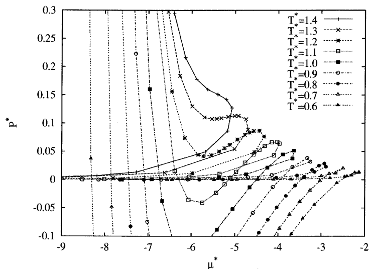
FIGURE 5.9: Pressure versus chemical potential (up to an additive constant) for a Lennard-Jones fluid, calculated on several isotherms using the HNC/H2 approximation.
