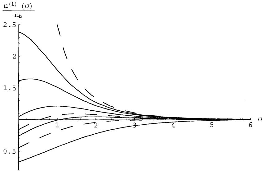
FIGURE 8.3: The density profile n^{(1)}(\sigma) (in units of n_b ) as a function of the distance from the boundary \sigma (in units of a ) for different values of the parameter g = \zeta/n_b in the case 4\pi n_b a^2 = 1 . From bottom to top, in full line g = 0.5, 1.5, 2.5, 5.0, 10.0 and in dashed line g = 1 (change of behavior between monotonous increasing profile and oscillating profile), g = 1.80237 (globally neutral system) and g \rightarrow \infty .
