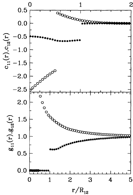
FIGURE 7.7: Monte Carlo results at a density \rho = \rho_1 = \rho_2 = 0.65/R_{12}^3 for the partial direct correlation function (on top) and the partial pair distribution function (below) of a mixture of non additive hard spheres with R_{11} = R_{22} = R_{12}/2 . The open circles denote the like correlation functions. The closed circles denote the unlike correlation functions.
