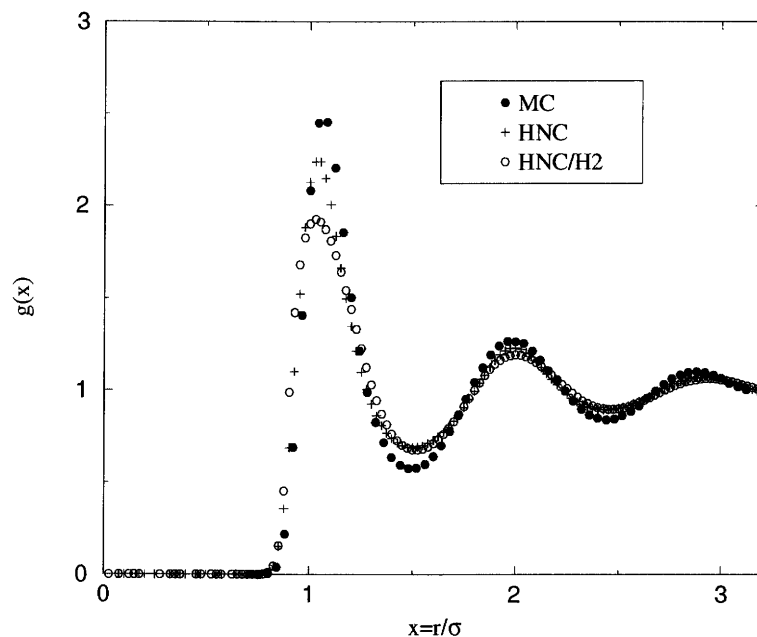
FIGURE 5.6: Comparison of the Monte Carlo (MC), HNC, and HNC/H2 results for the pair distribution function of the inverse 4th-power fluid at z = 3.92 .
