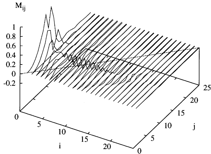
FIGURE 6.4: We show a surface plot of the Floquet matrix (6.ii:7) calculated for three dimensional hard spheres in HNC approximation at \eta = 0.3 . The matrix was generated using N = 256 grid points but only the region significantly different from zero is shown.
