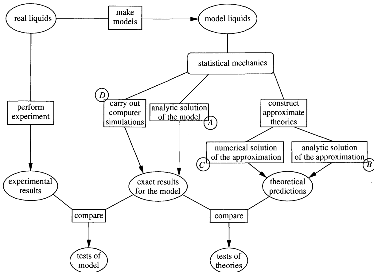
FIGURE 2.2: Block diagram showing the processes needed to test a particular model of a liquid and the ones needed to test a particular theory for a given model. In the thesis we will present some examples to illustrate those parts of the diagram which have a circle beneath them.
