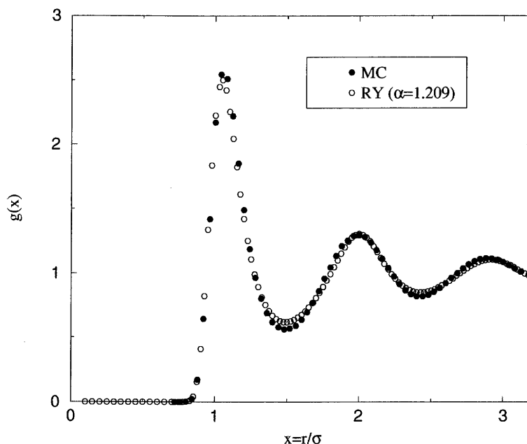
FIGURE 5.3: Comparison of the Monte Carlo (MC) and Rogers Young (RY) results for the pair distribution function of the inverse 6th-power fluid at z = 1.54 .
