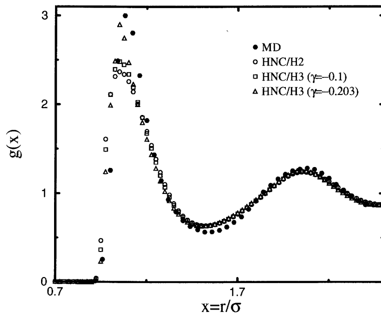
FIGURE 5.11: Comparison of the pair distribution function of a Lennard-Jones fluid at \rho^* = 0.85 and T^* = 0.719 computed from the molecular dynamic (MD) simulation of Verlet, the HNC/H2 approximation, and the HNC/H3 approximation. For HNC/H3 we present results obtained setting \gamma = -0.1 (when the generating functional of the approximation is still strictly convex) and \gamma = -0.203 (which gives the best fit possible to the simulation data but does not ensure the strict convexity of the generating functional).
