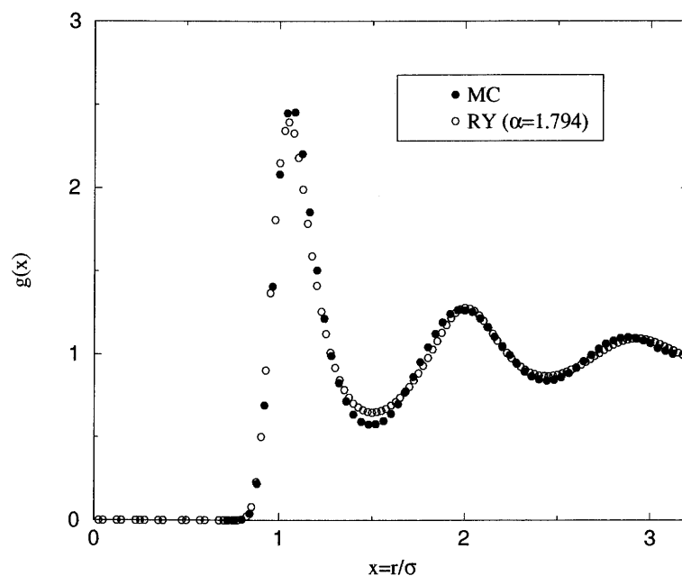
FIGURE 5.5: Comparison of the Monte Carlo (MC) and Rogers Young (RY) results for the pair distribution function of the inverse 4th-power fluid at z = 3.92 .
