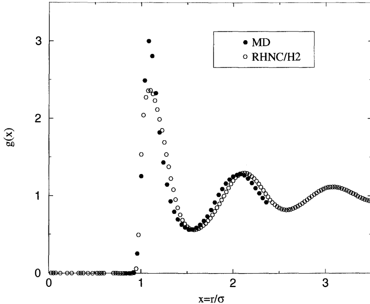
FIGURE 5.10: Comparison of the pair distribution function computed from the RHNC/H2 with a yukawian G function and from a molecular dynamics (MD) simulation, for a Lennard-Jones fluid at \rho^* = 0.85 and T^* = 0.719 .
