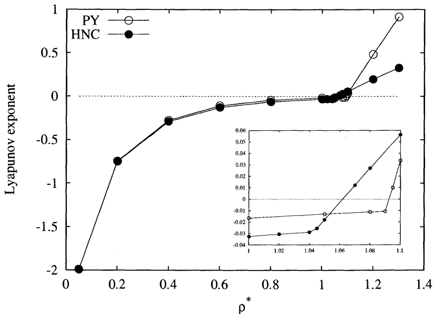
FIGURE 6.2: We show the Lyapunov exponent as a function of the reduced density for a Lennard-Jones fluid at a reduced temperature T^* = 2.74 as calculated using the PY and the HNC closures.
