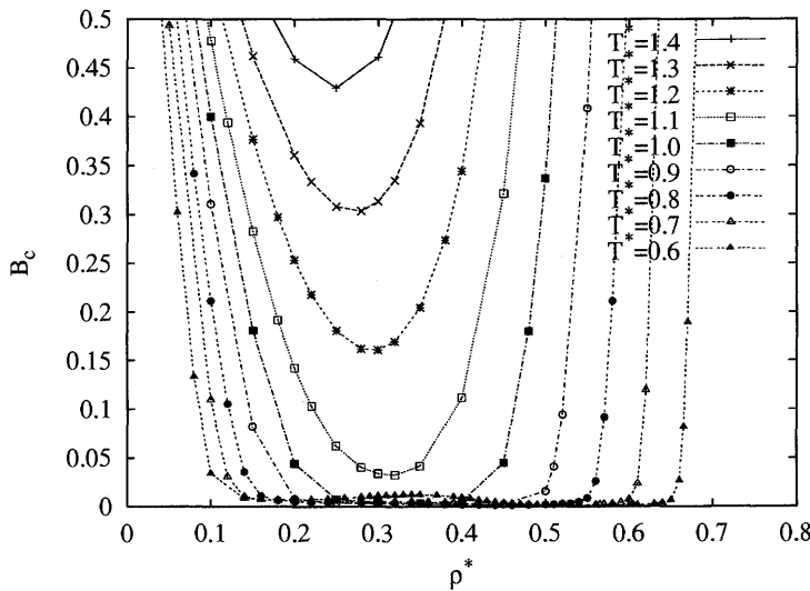
FIGURE 5.7: Behavior of B_c of the Lennard-Jones fluid, on several isotherms as a function of the density for the HNC/H2 approximation.
