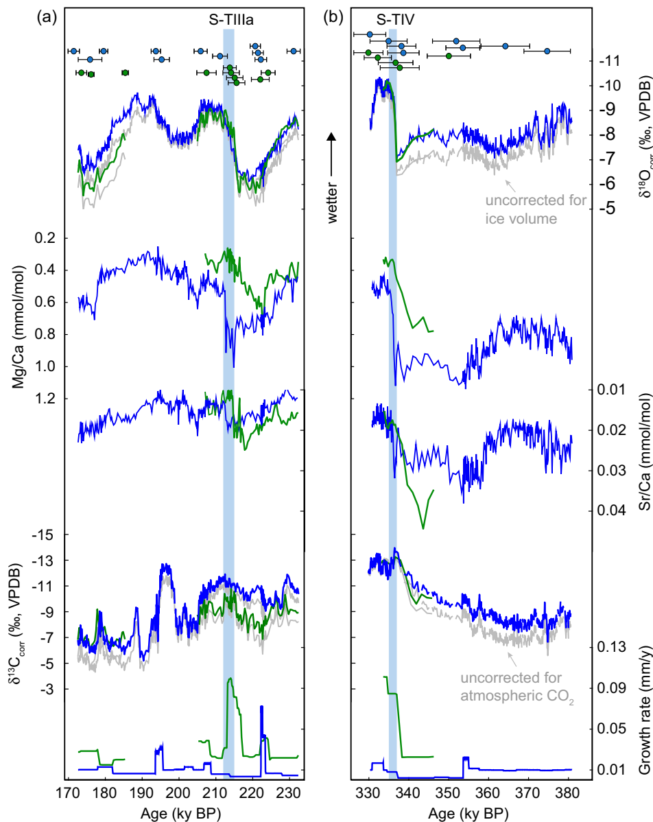
Fig. 3 Stalagmite \delta^{18}\text{O} , Mg/Ca, Sr/Ca, \delta^{13}\text{C} and growth rates. a Stalagmites AC11-06 and AC11-03 spanning Sulawesi termination IIIa (S-TIIIa) and b AC09-04 and AC11-02 spanning Sulawesi termination IV (S-TIV). Geochemical data for fast-growing stalagmites (AC11-03, AC11-02) are shown in green, slow-growing stalagmites (AC11-06, AC09-04) are shown in blue. Stalagmite \delta^{18}\text{O} has been corrected for the effect of ice volume 45 and stalagmite \delta^{13}\text{C} has been corrected for the effect of atmospheric \text{CO}_2 53 ; the uncorrected records are shown in grey (see Supplementary Methods for details of these corrections). Sulawesi glacial terminations (determined by prominent shifts in Sulawesi stalagmite \delta^{18}\text{O} , Supplementary Methods) are indicated by blue bars. Colour-coded circles at the top of each panel show U-Th dates and their uncertainties ( 2\sigma ). The y axes for geochemical profiles are inverted to show wetter conditions upward.
